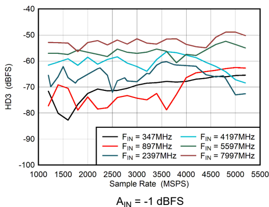
Figure 6-53. Dual Channel Mode: HD3 vs Sample Rate
