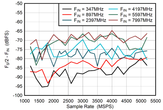
Figure 6-56. Dual Channel Mode: F_S/2 - F_{\text{IN}} vs Sample Rate
