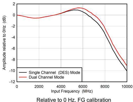
Figure 6-1. Input Amplitude vs Input Frequency
