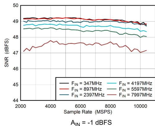
Figure 6-29. DES Mode: SNR vs Sample Rate
