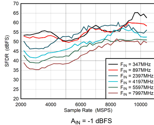
Figure 6-32. DES Mode: SFDR vs Sample Rate
