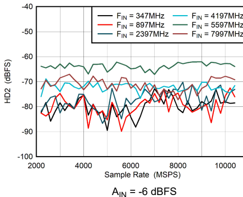
Figure 6-36. DES Mode: HD2 vs Sample Rate
