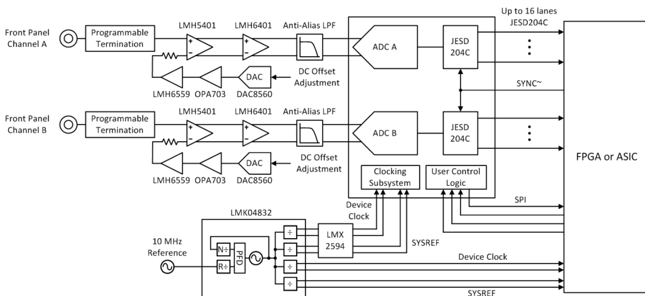
Figure 8-1. Typical Configuration for Reconfigurable Oscilloscope
