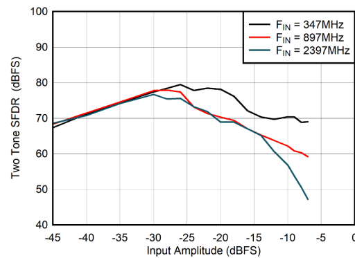
Figure 6-104. DES Mode: Two Tone SFDR vs Input Amplitude
