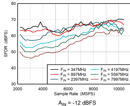
Figure 6-34. DES Mode: SFDR vs Sample Rate
