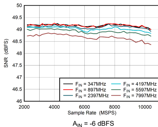
Figure 6-30. DES Mode: SNR vs Sample Rate
