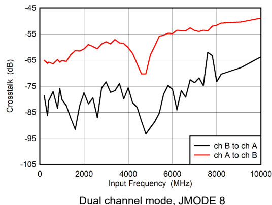
Figure 6-2. Crosstalk vs Input Frequency
