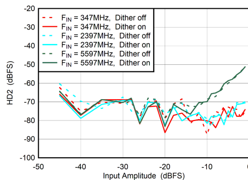
Figure 6-76. Dual Channel Mode: HD2 vs Input Amplitude and Dither
