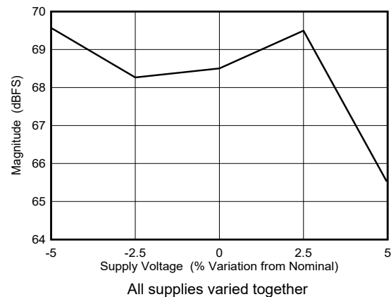
Figure 6-96. Dual Channel Mode: SFDR vs Supply Voltage
