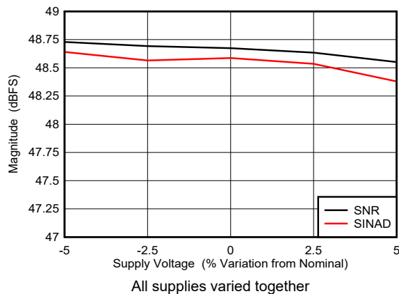
Figure 6-95. Dual Channel Mode: SNR and SINAD vs Supply Voltage
