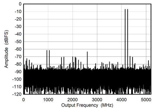
Figure 6-14. DES Mode: Two Tone FFT at 4197 MHz
