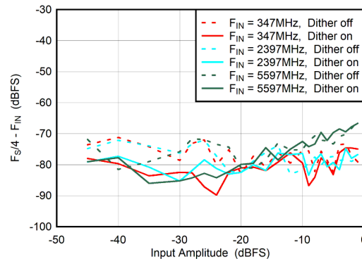
Figure 6-70. DES Mode: F_S/4 - F_{\text{IN}} vs Input Amplitude and Dither
