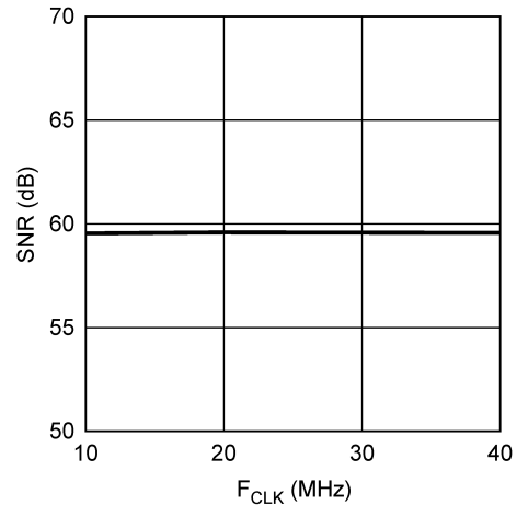
Figure 13. SNR vs. f_{CLK}
