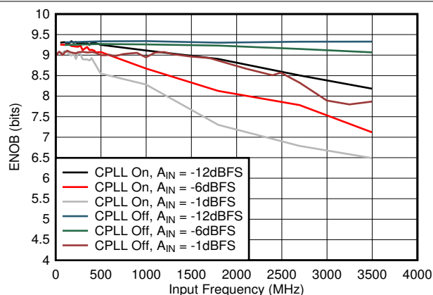
图 8-51. ENOB vs A_{IN} and C-PLL
