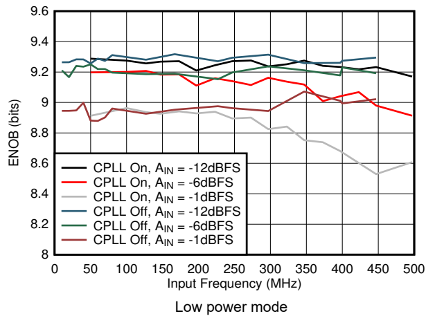
图 8-57. ENOB vs A_{IN} and C-PLL
