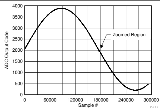
图 8-124. Background Calibration Core Transition (midscale voltage)
