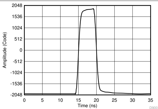
图 10-2. Measured Pulse using Sub-Sampling Technique for Equivalent 32 GSPS Measurement
