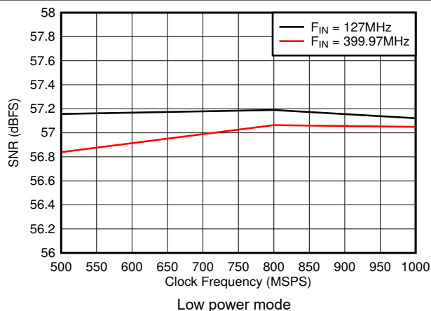
图 8-28. SNR vs Sample Rate
