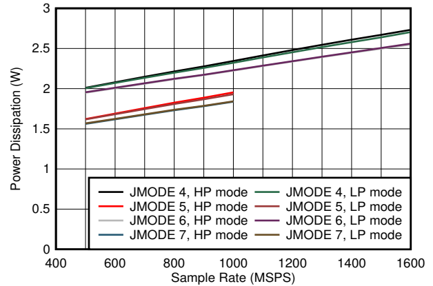
图 8-80. Quad Channel, Power Dissipation vs F_s and JMODE 4 - 7
