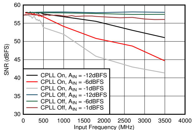
图 8-49. SNR vs A_{IN} and C-PLL
