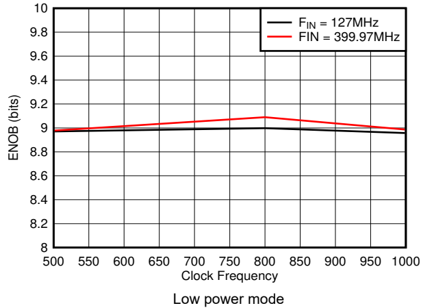
图 8-31. ENOB vs Sample Rate
