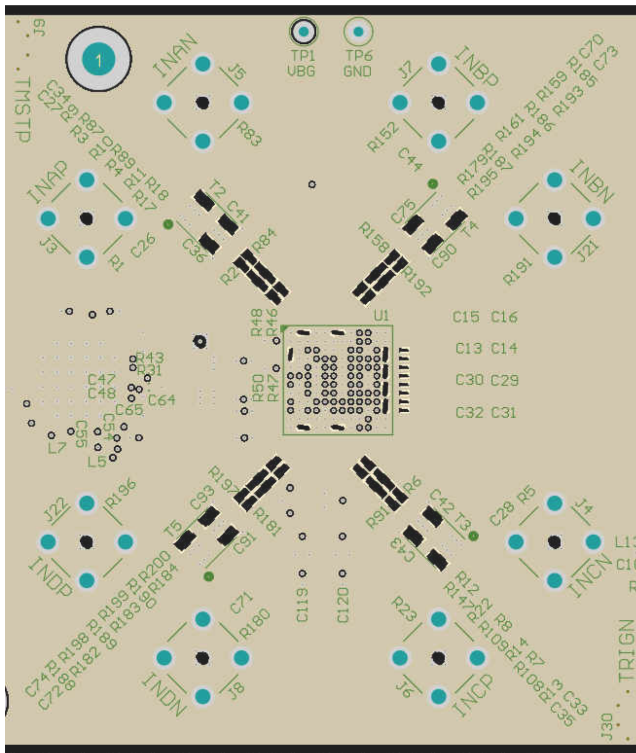
图 12-2. GND1 Cutouts to Optimize Impedance of Component Pads
