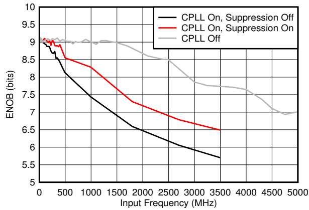
图 8-43. ENOB vs F_{IN} and C-PLL modes
