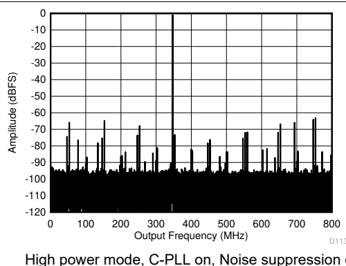
图 8-6. Single Tone FFT at 347 MHz and -1 dBFS
