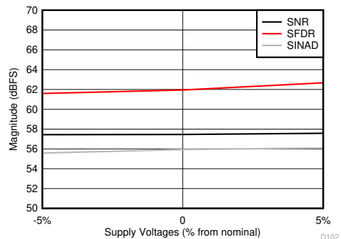
图 8-62. SNR, SFDR and SINAD vs Supply Voltages
