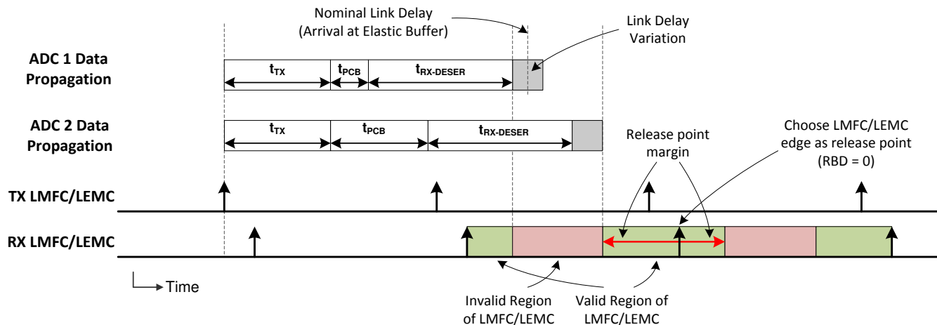
图 9-11. LMFC/LEMC Valid Region Definition for Elastic Buffer Release Point Selection
