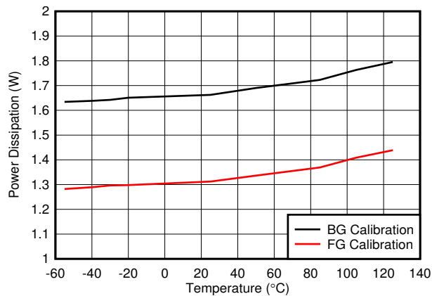
图 8-121. Quad Channel, Power Dissipation vs Temperature
