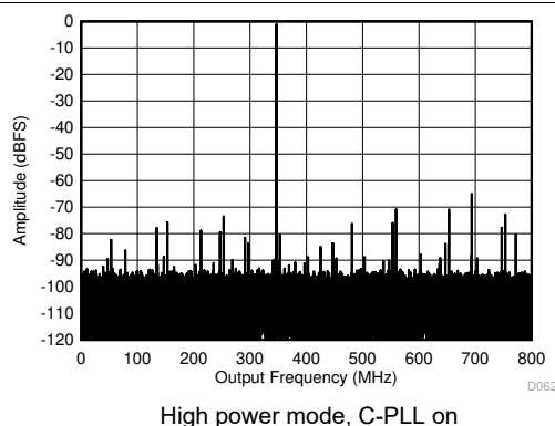
图 8-5. Single Tone FFT at 347 MHz and -1 dBFS
