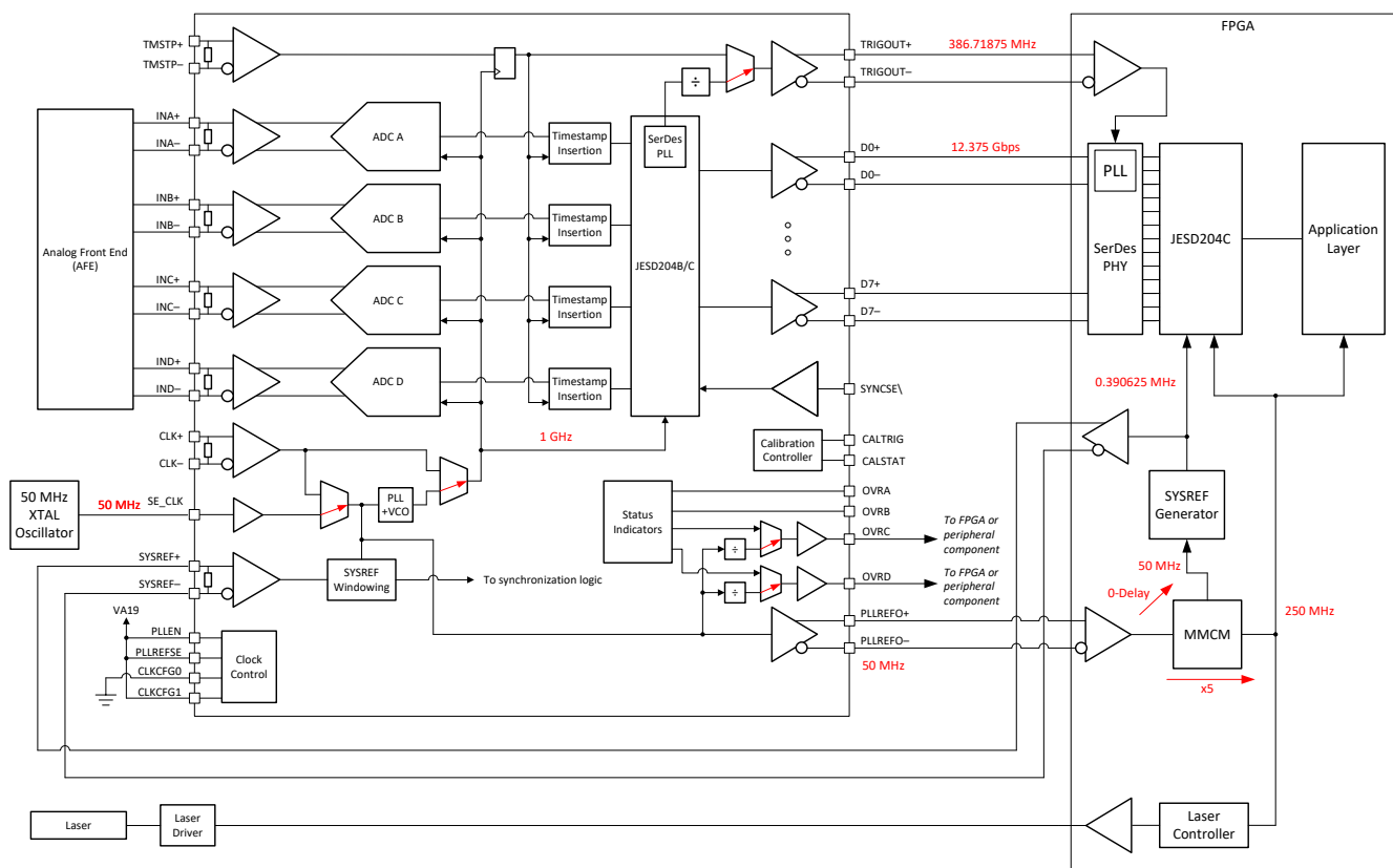
图 10-1. Typical Configuration for a LiDAR Digitizer
