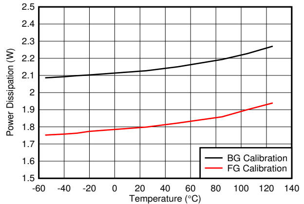
图 8-122. Dual Channel, Power Dissipation vs Temperature
