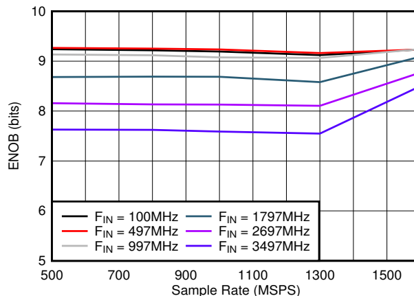
图 8-26. ENOB vs Sample Rate
