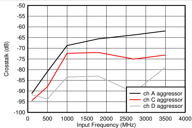
图 8-78. Crosstalk to Channel B vs F_{IN}
