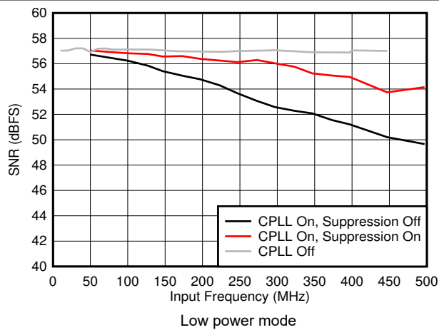
图 8-45. SNR vs F_{IN} and C-PLL modes
