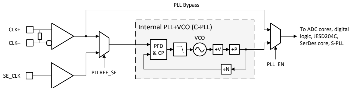
图 9-6. Converter PLL (C-PLL) Architecture
