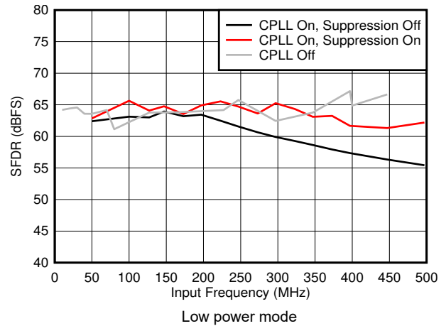
图 8-44. SFDR vs F_{IN} and C-PLL modes
