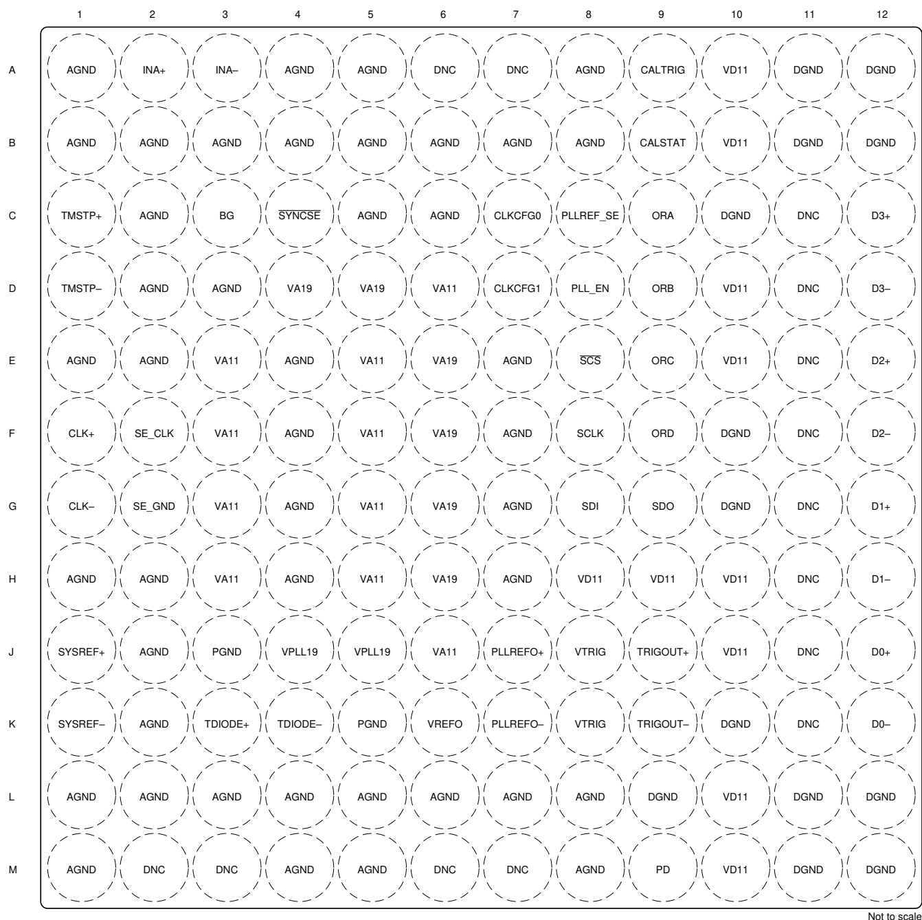
图 7-3. Single Channel AAV Package, 144-Ball Flip Chip BGA (Top View)
