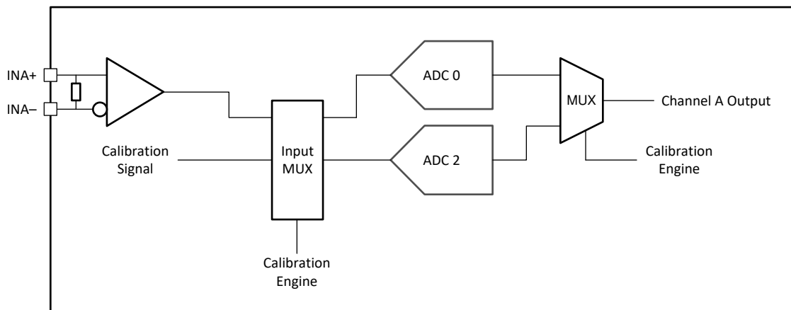
图 9-17. Single Channel Calibration System Block Diagram
