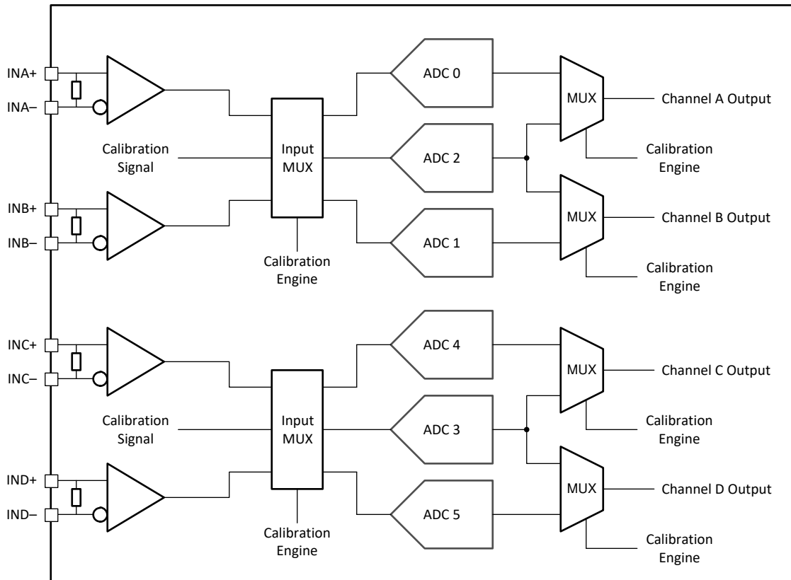
图 9-15. Quad Channel Calibration System Block Diagram
