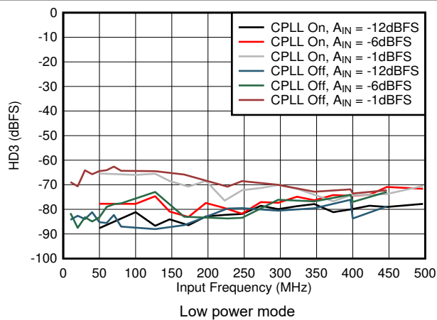
图 8-59. HD3 vs A_{IN} and C-PLL
