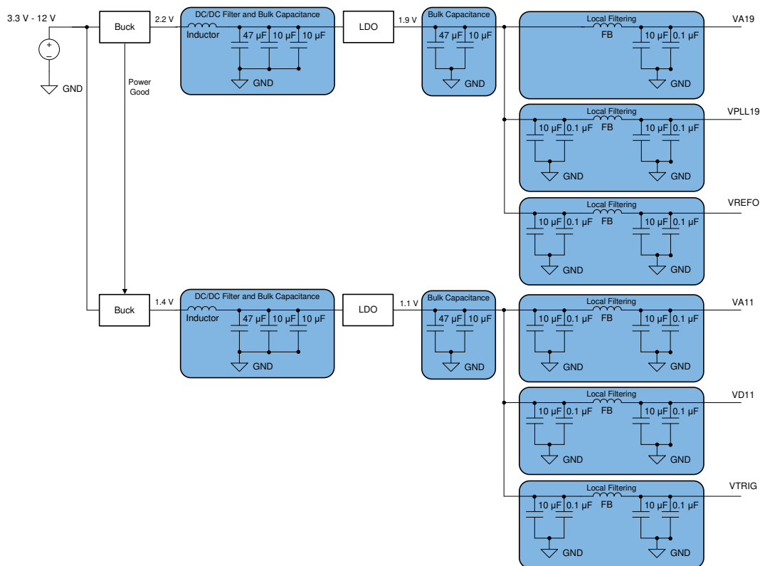
图 11-1. LDO Linear Regulator Approach Example
