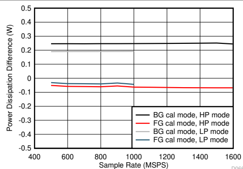
图 8-110. Dual Channel, Power Dissipation Change with Calibration Mode
