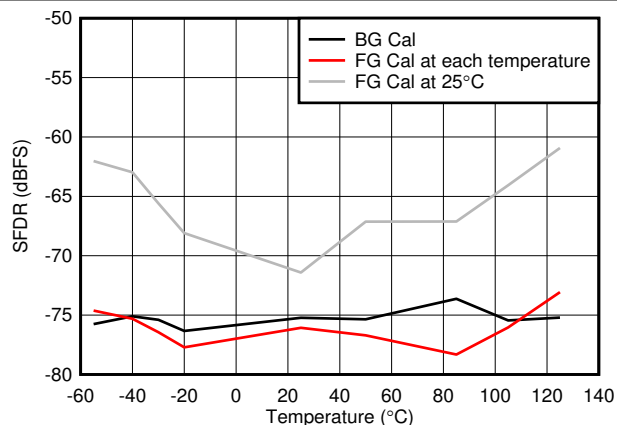
图 8-68. Worst Spur vs Temperature
