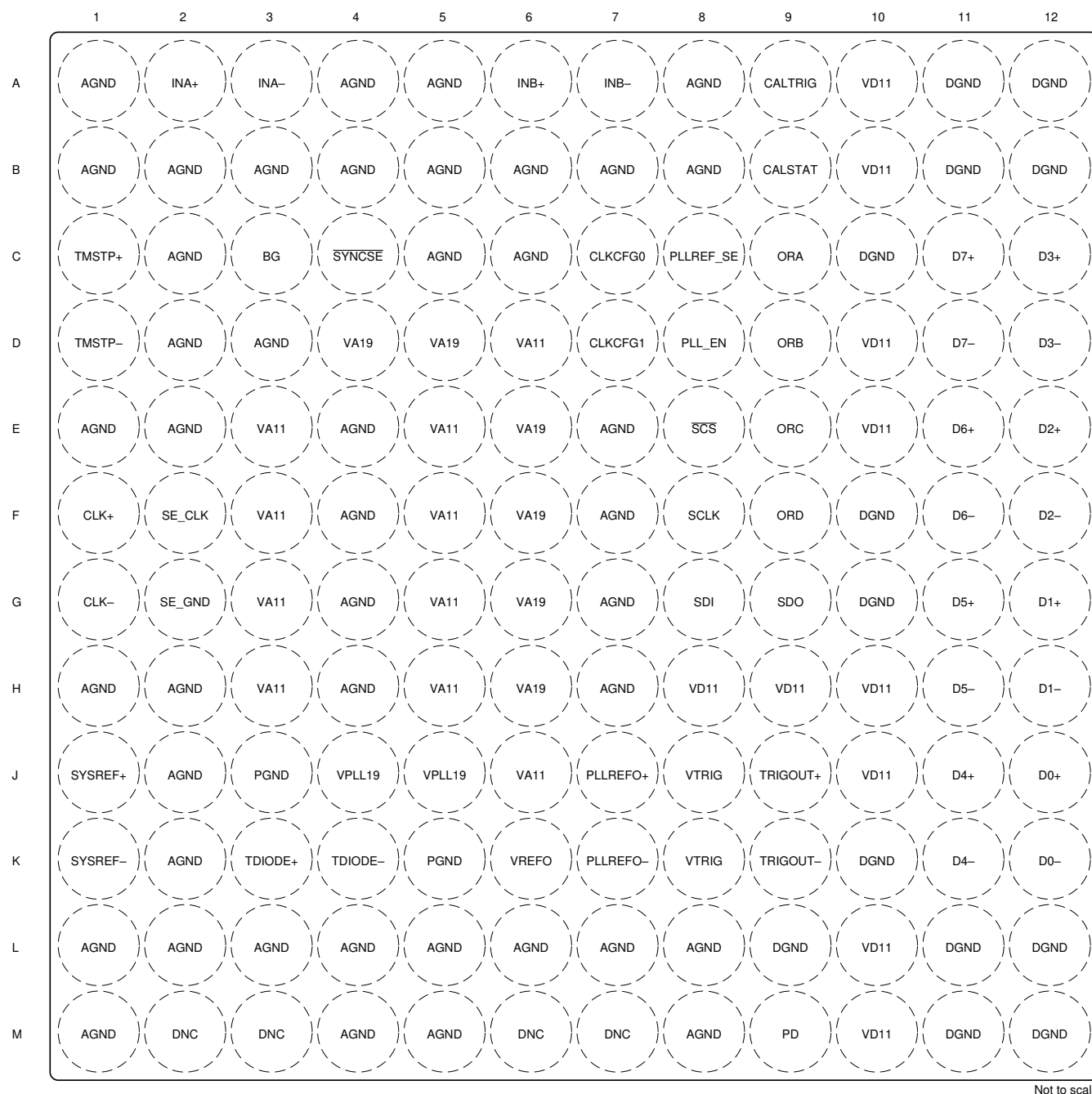
图 7-2. Dual Channel AAV Package, 144-Ball Flip Chip BGA (Top View)
