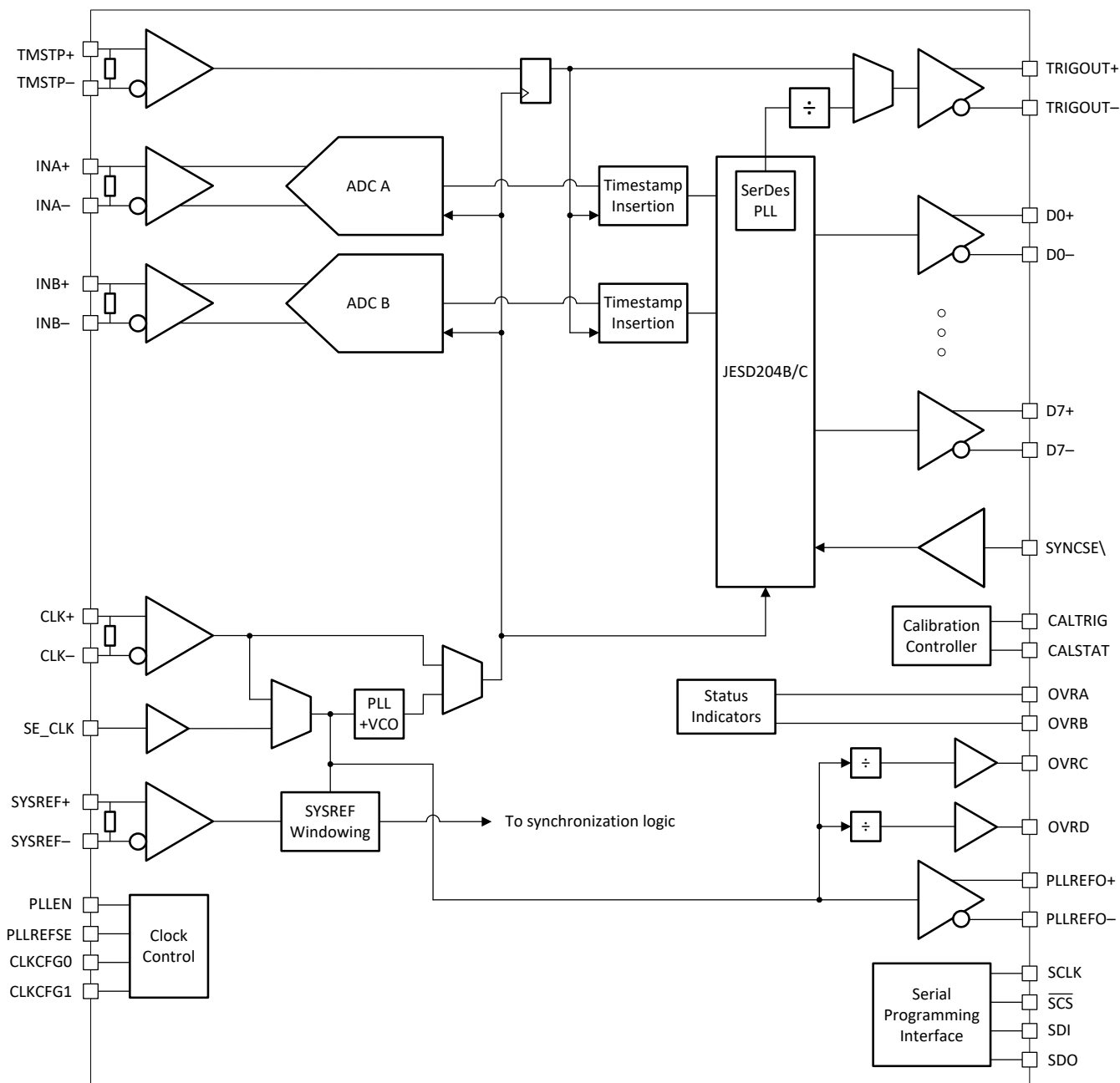
图 9-2. Dual Channel Functional Block Diagram
