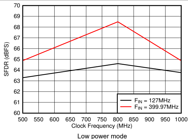
图 8-29. SFDR vs Sample Rate
