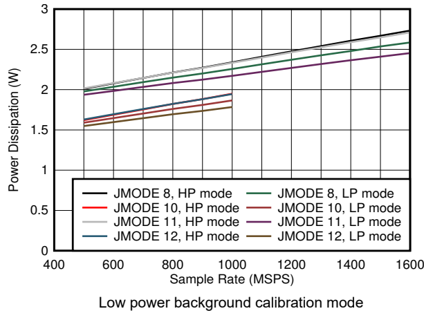
图 8-81. Quad Channel, Power Dissipation vs F_s and JMODE 8 - 12
