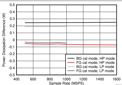
图 8-109. Quad Channel, Power Dissipation Change with Calibration Mode
