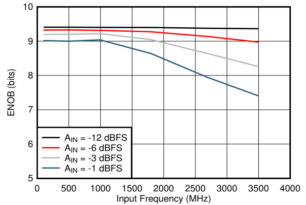
图 8-20. ENOB vs Input Frequency
