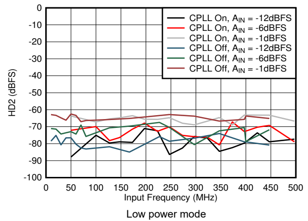
图 8-58. HD2 vs A_{IN} and C-PLL
