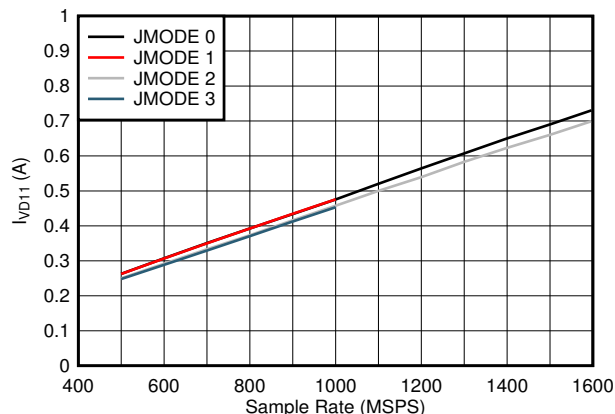
图 8-85. Quad Channel, I_{VD11} vs F_S and JMODE 0 - 3
