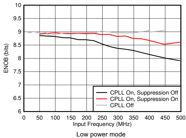
图 8-47. ENOB vs F_{IN} and C-PLL modes
