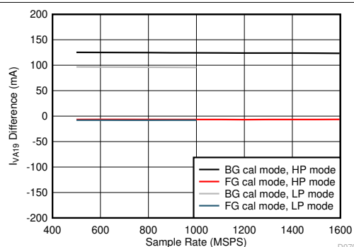
图 8-112. Quad Channel, I_{VA19} Change with Calibration Mode
