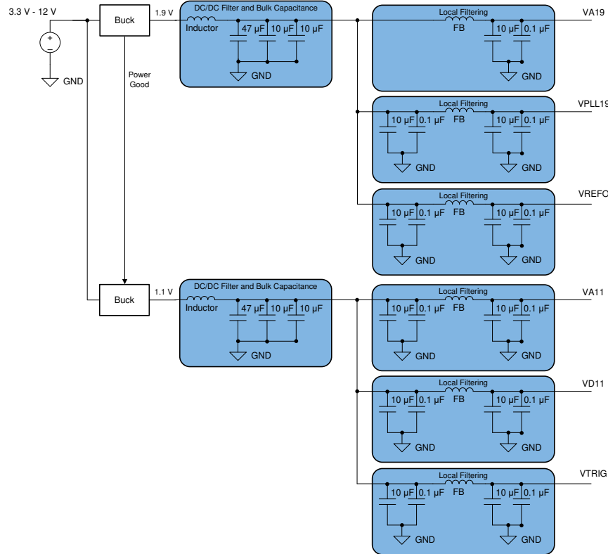
图 11-2. Switcher-Only Approach Example
