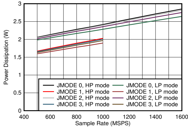
图 8-79. Quad Channel, Power Dissipation vs F_s and JMODES 0 - 3
