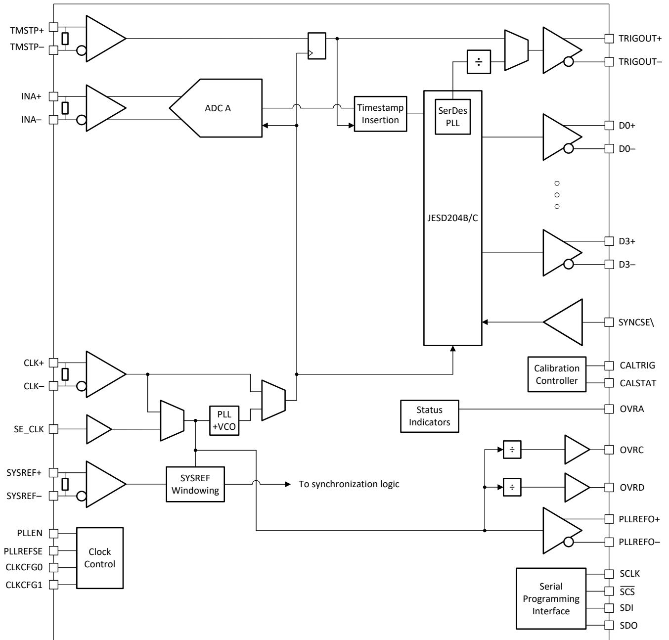
图 9-3. Single Channel Functional Block Diagram
