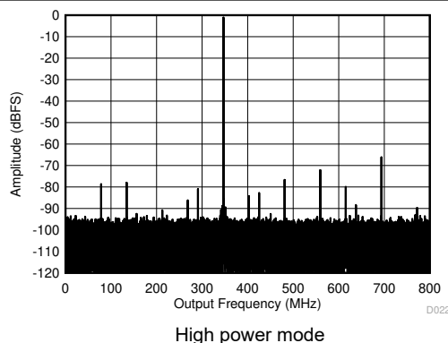
图 8-4. Single Tone FFT at 347 MHz and -1 dBFS
