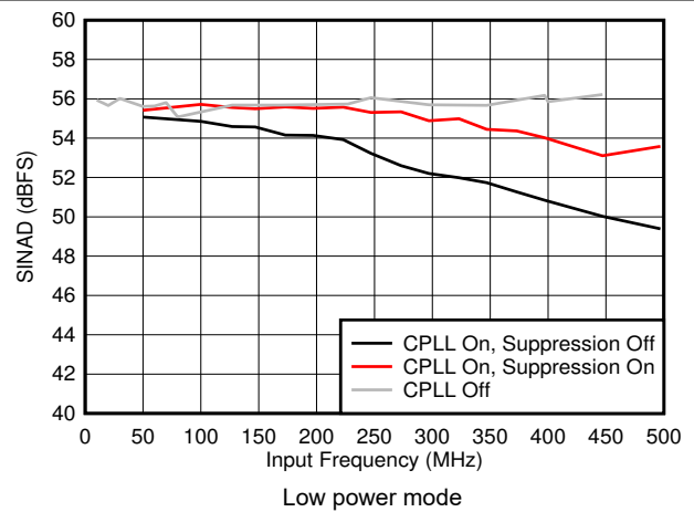
图 8-46. SINAD vs F_{IN} and C-PLL modes
