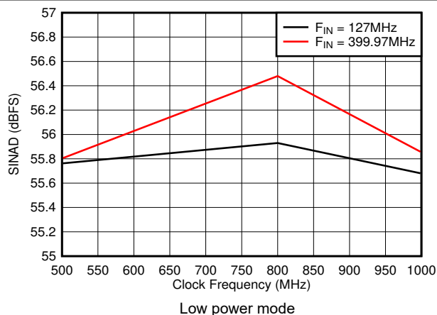
图 8-30. SINAD vs Sample Rate
