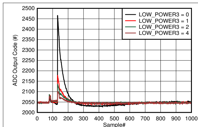
图 9-12. Background Calibration Core Transition In Low Power Mode
