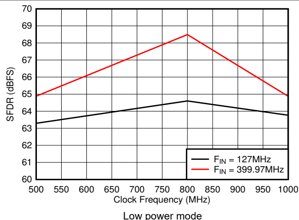
图 8-27. SFDR vs Sample Rate
