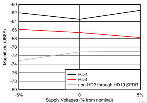
图 8-61. HD2, HD3 and Worst non-HD Spur vs Supply Voltage
