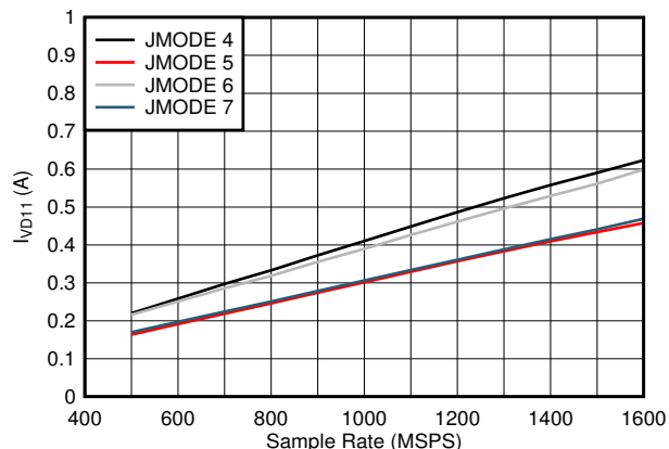
图 8-86. Quad Channel, I_{VD11} vs F_S and JMODE 4 - 7
