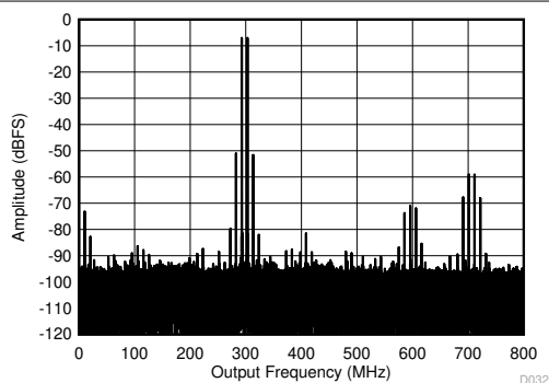
图 8-69. Two Tone FFT at 498MHz
