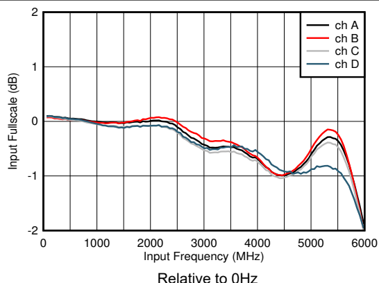
图 8-3. Input Fullscale vs Frequency
