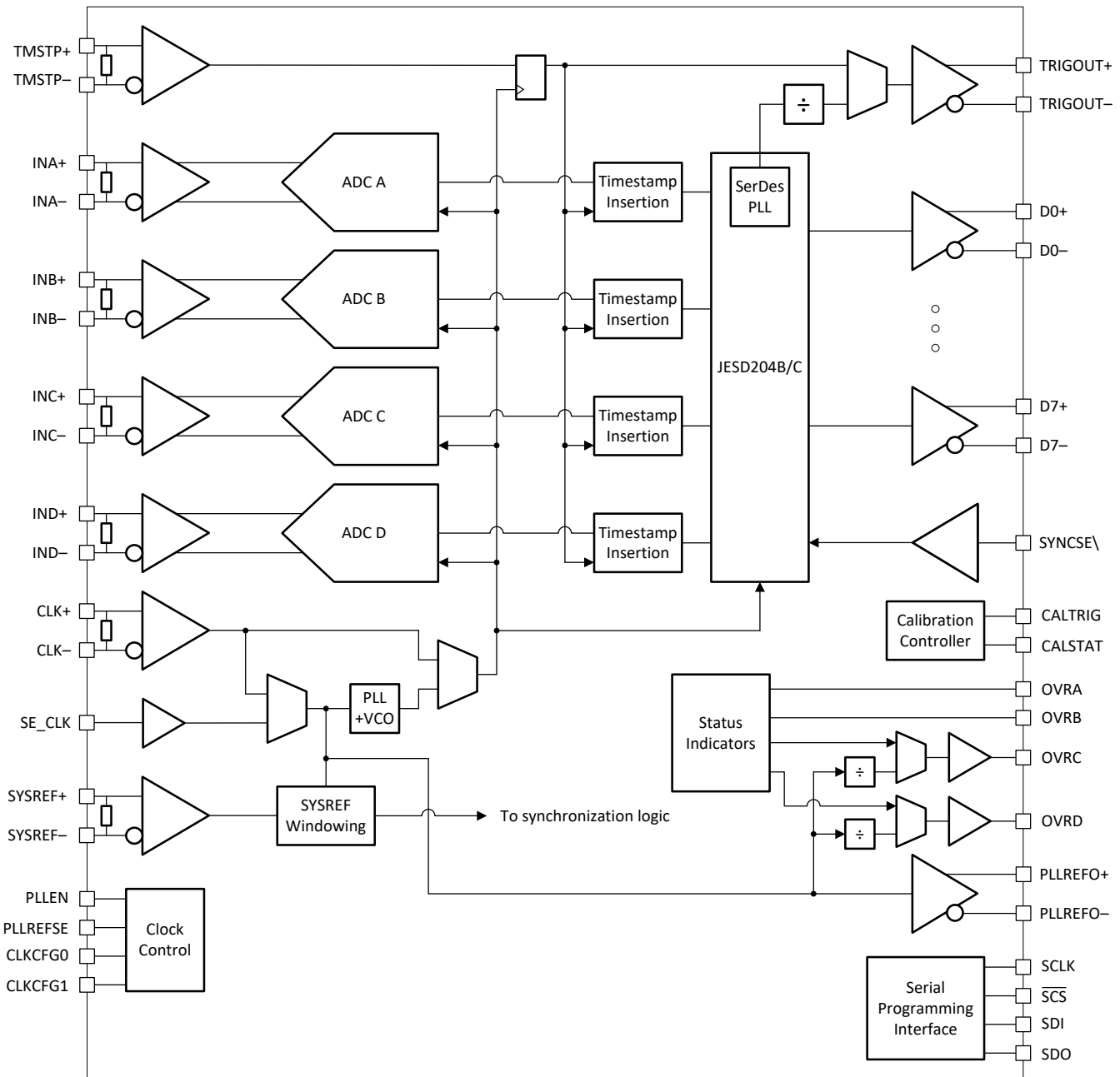
图 9-1. Quad Channel Functional Block Diagram
