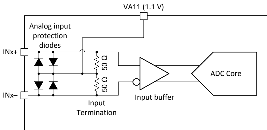
图 9-4. Analog Input Internal Termination and Protection Diagram
