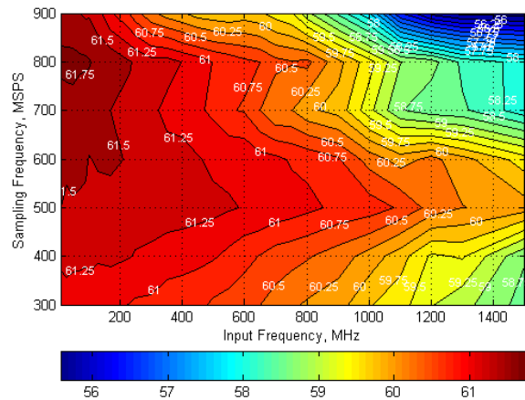
图 35. SNR Across Input and Sampling Frequencies (Auto On)
