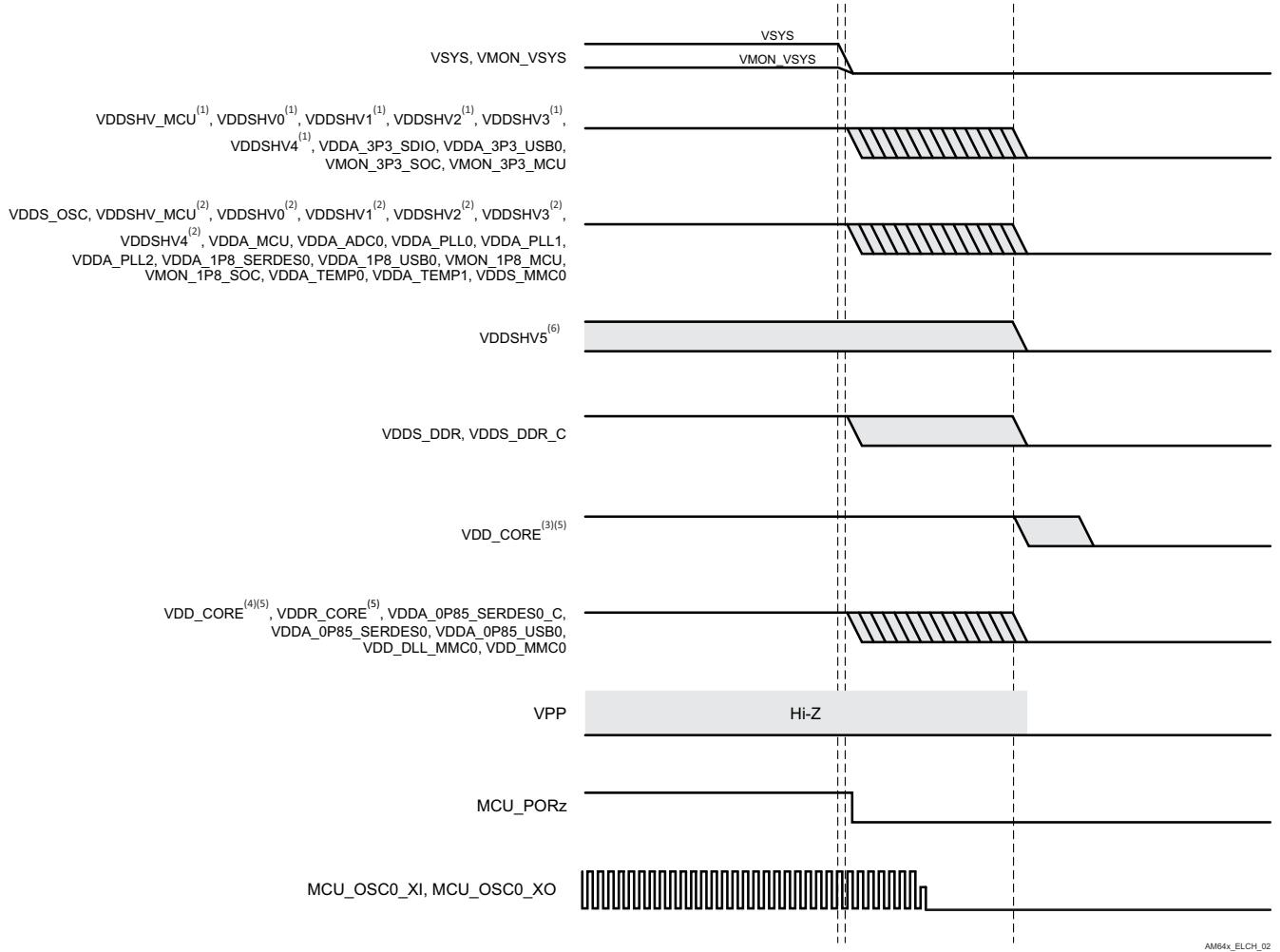
图 7-6. Power-Down Sequencing
