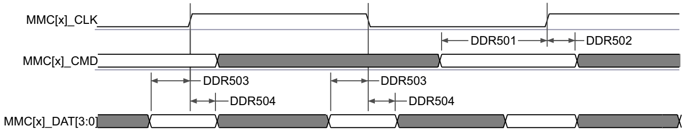
图 7-74. MMC1 – UHS-I DDR50 – Receive Mode
