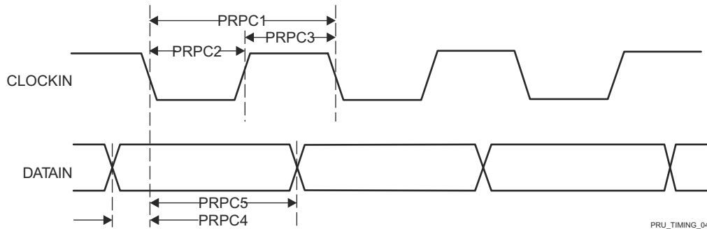
图 7-92. PRU_ICSSG PRU Parallel Capture Timing Requirements – Falling Edge Mode
