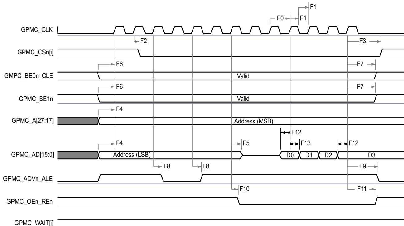
图 7-41. GPMC and NOR Flash—Synchronous Burst Write (GPMCFCLKDIVIDER = 0)
