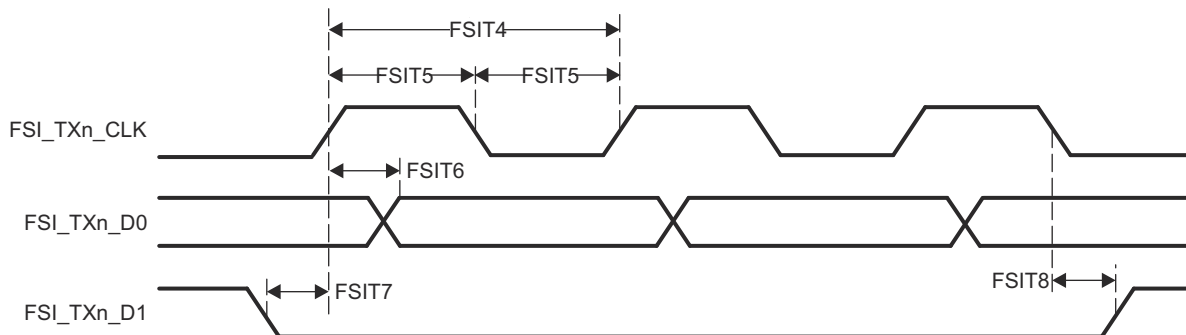
图 7-38. FSI Switching Characteristics - SPI Mode
