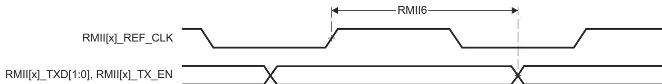
图 7-25. RMII[x]_TXD[1:0], and RMII[x]_TX_EN Switching Characteristics - RMII Mode
