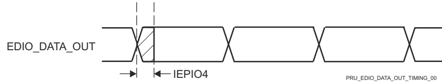
图 7-101. PRU_ICSSG IEP Digital IOs Timing Requirements
