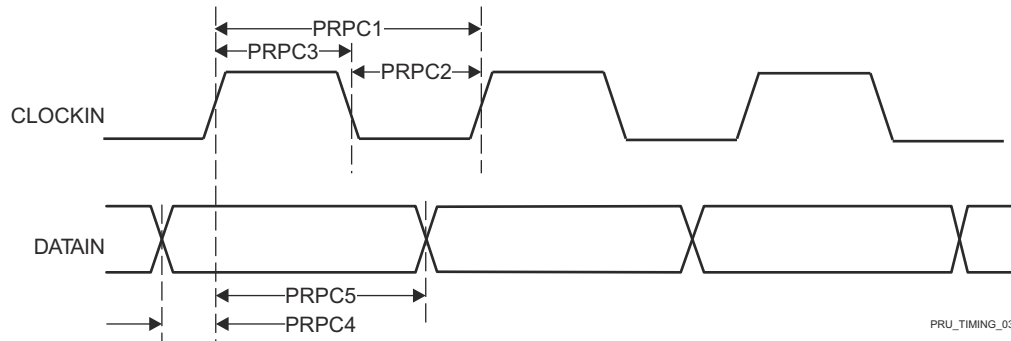
图 7-91. PRU_ICSSG PRU Parallel Capture Timing Requirements – Rising Edge Mode
