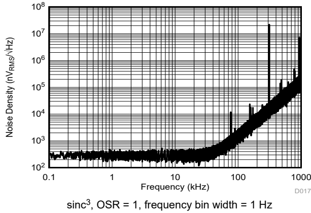
图 6-24. Noise Density With Both Inputs Shorted to HGND
