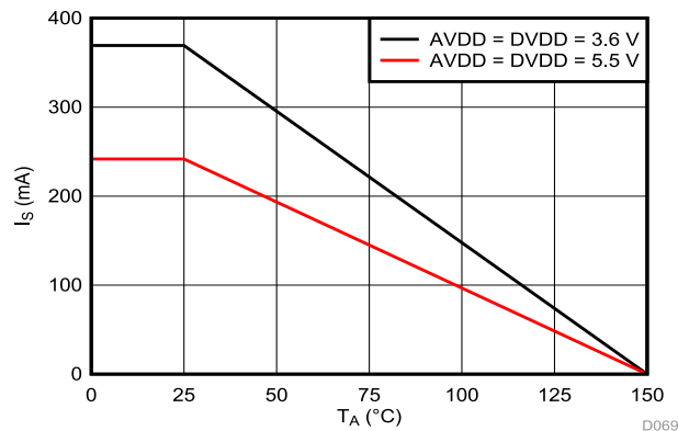
6-3. Thermal Derating Curve for Safety-Limiting Current per VDE
