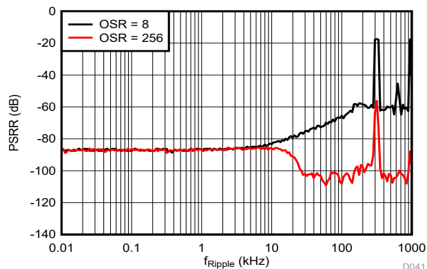
图 6-13. Power-Supply Rejection Ratio vs Ripple Frequency
