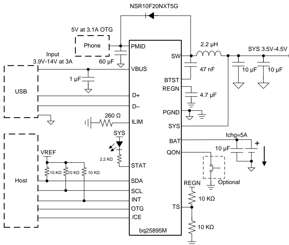
图 58. bq25895M with D+/D- Interface, 3.1 A Boost Mode Output, and no Thermistor Connections
