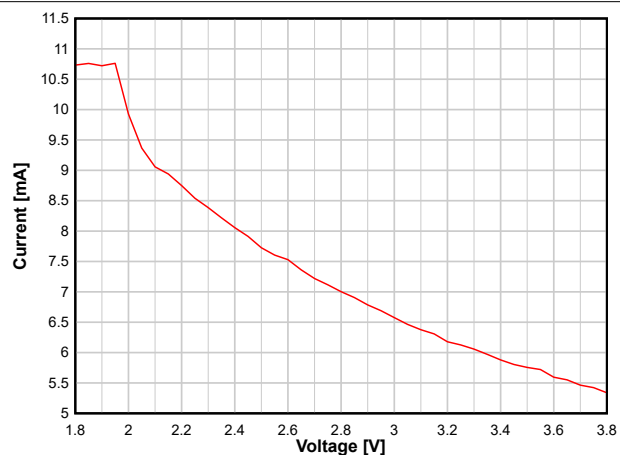
图 8-8. RX Current versus Supply Voltage (VDD5) (BLE 1 Mbps, 2.44 GHz)
