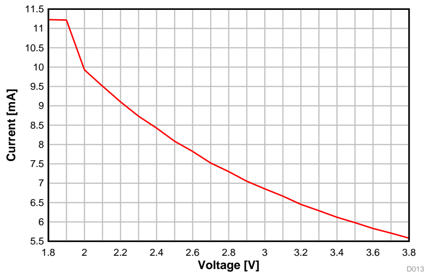
图 5-8. RX Current vs. Supply Voltage (VDD5) (BLE 1 Mbps, 2.44 GHz)
