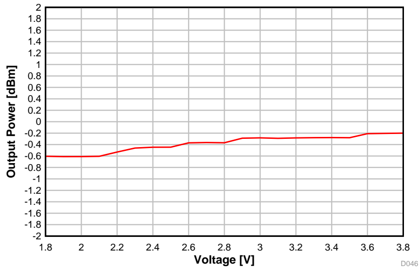
图 5-17. Output Power vs. Supply Voltage (VDD5) (BLE 1 Mbps, 2.44 GHz)
