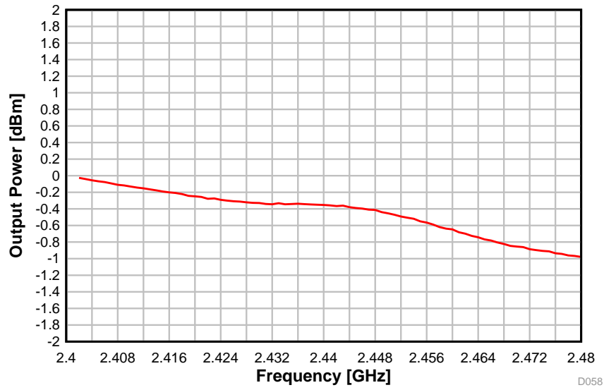
图 5-19. Output Power vs. Frequency (BLE 1 Mbps, 2.44 GHz)
