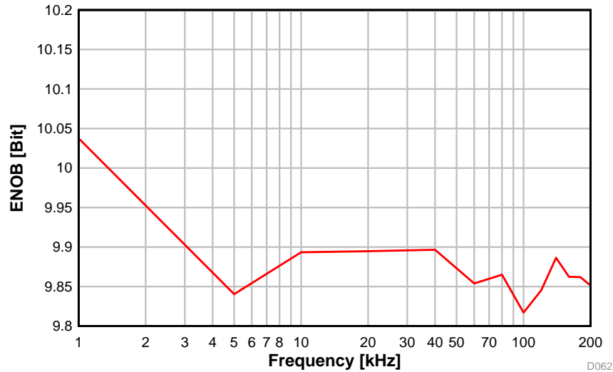
图 5-22. ENOB vs. Sampling Frequency
