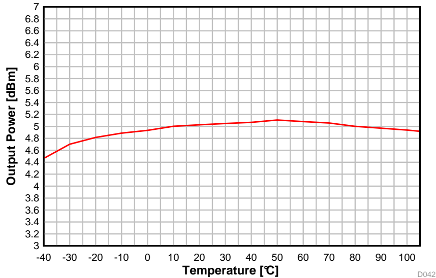
图 5-16. Output Power vs. Temperature (BLE 1 Mbps, 2.44 GHz, +5 dBm)
