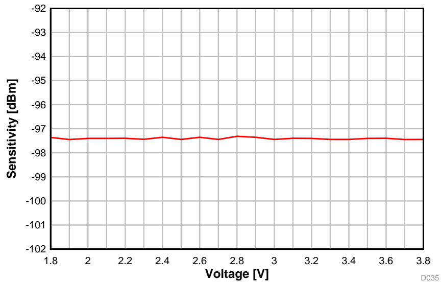
图 5-14. Sensitivity vs. Supply Voltage (VDDS) (BLE 1 Mbps, 2.44 GHz, DCDC Off)
