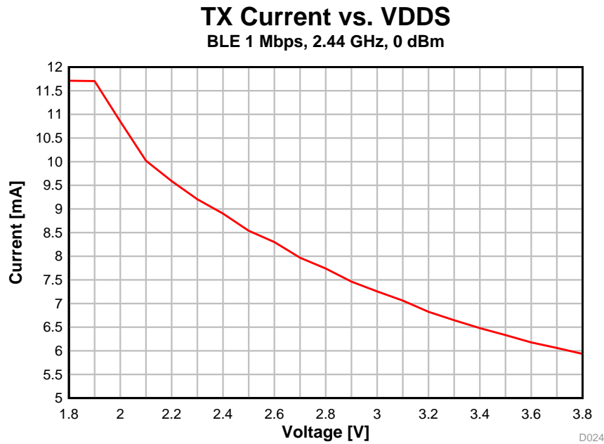
图 5-10. TX Current vs. Supply Voltage (VDDS) (BLE 1 Mbps, 2.44 GHz)
