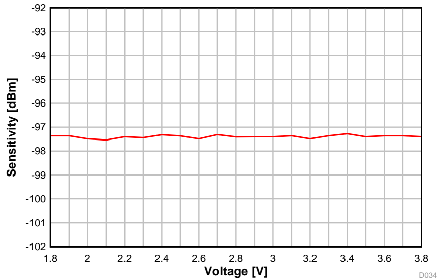
图 5-13. Sensitivity vs. Supply Voltage (VDDS) (BLE 1 Mbps, 2.44 GHz)
