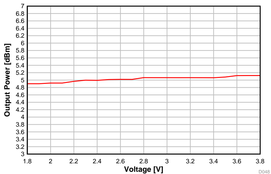
图 5-18. Output Power vs. Supply Voltage (VDD5) (BLE 1 Mbps, 2.44 GHz, +5 dBm)
