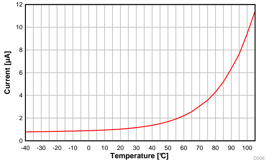
图 5-5. Standby Mode (MCU) Current vs. Temperature
