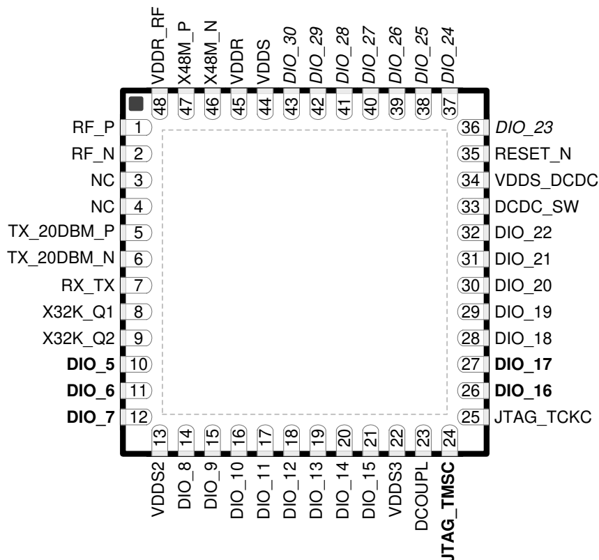
图 7-1. RGZ (7-mm x 7-mm) Pinout, 0.5-mm Pitch (Top View)
