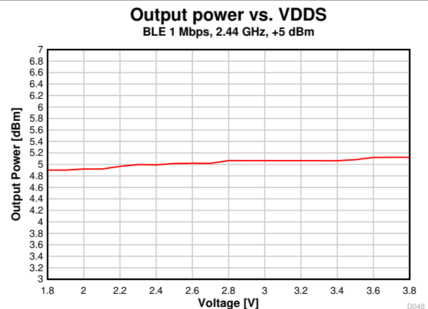
图 8-26. Output Power vs. Supply Voltage (VDD5) (BLE 1 Mbps, 2.44 GHz, +5 dBm)
