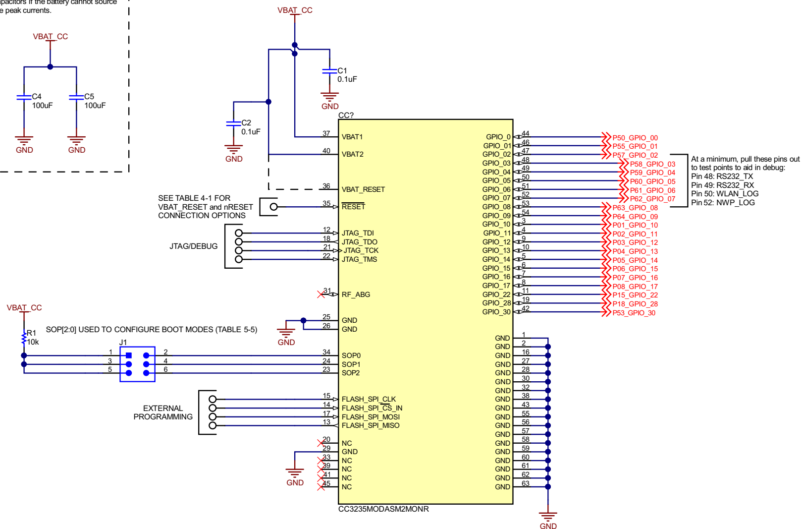
图 10-4. CC3235MODx Typical Application Schematic
