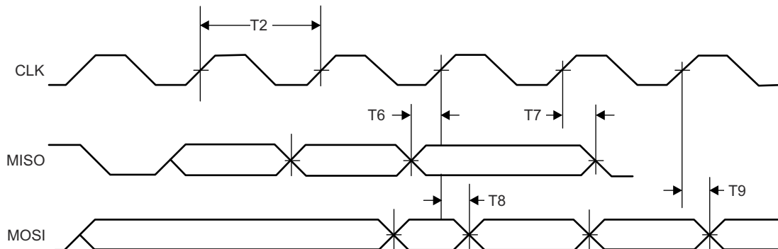
图 8-8. SPI Master Timing Diagram
