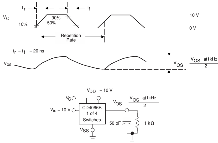
Figure 13. Propagation Delay, t_{PLH} , t_{PHL} Control-Signal Output
