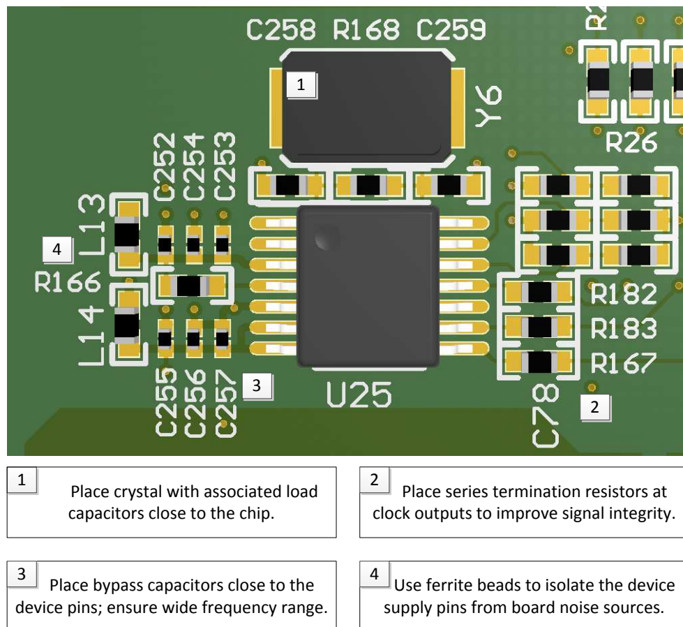
Figure 23. Annotated Layout
