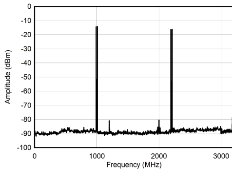
图 6-31. Dual Channel RTZ Mode: Dual Tone Spectrum at 1 GHz \pm 10 MHz
