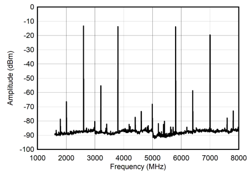
图 6-34. Dual Channel 2xRF Mode: Single Tone Spectrum at 3.8 to 5.8 GHz
