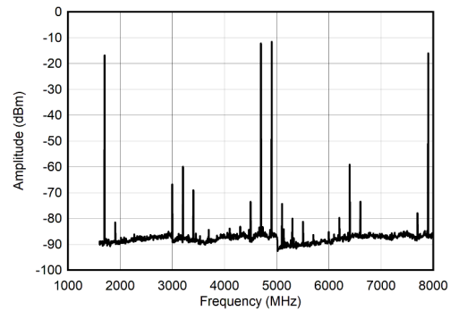
图 6-36. Dual Channel 2xRF Mode: Single Tone Spectrum at 4.7 to 4.9 GHz
