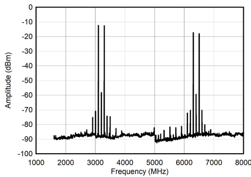
图 6-33. Dual Channel 2xRF Mode: Single Tone Spectrum at 3.3 to 6.3 GHz
