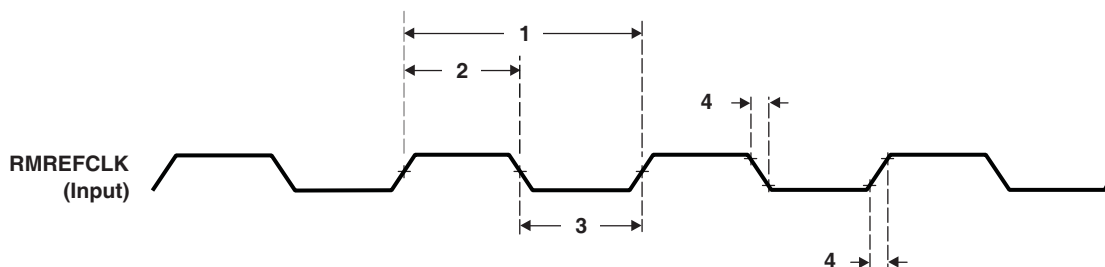
Figure 8-14. RMREFCLK Timing RMII Operation
