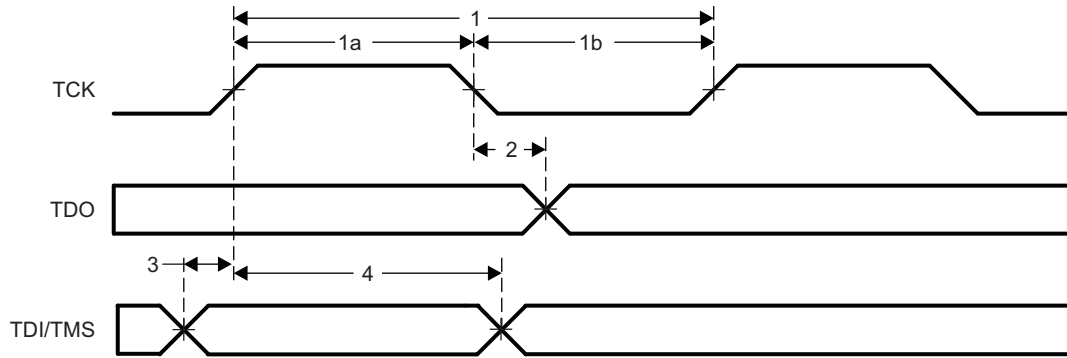
Figure 8-7. JTAG Timing
