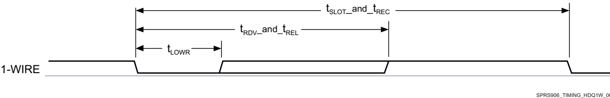
图 5-46. 1-Wire—Read Bit (Data)
