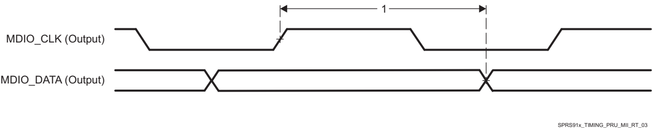
图 5-124. PRU-ICSS MDIO_DATA Timing – Output Mode
