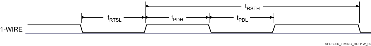
图 5-45. 1-Wire—Break (Reset)
