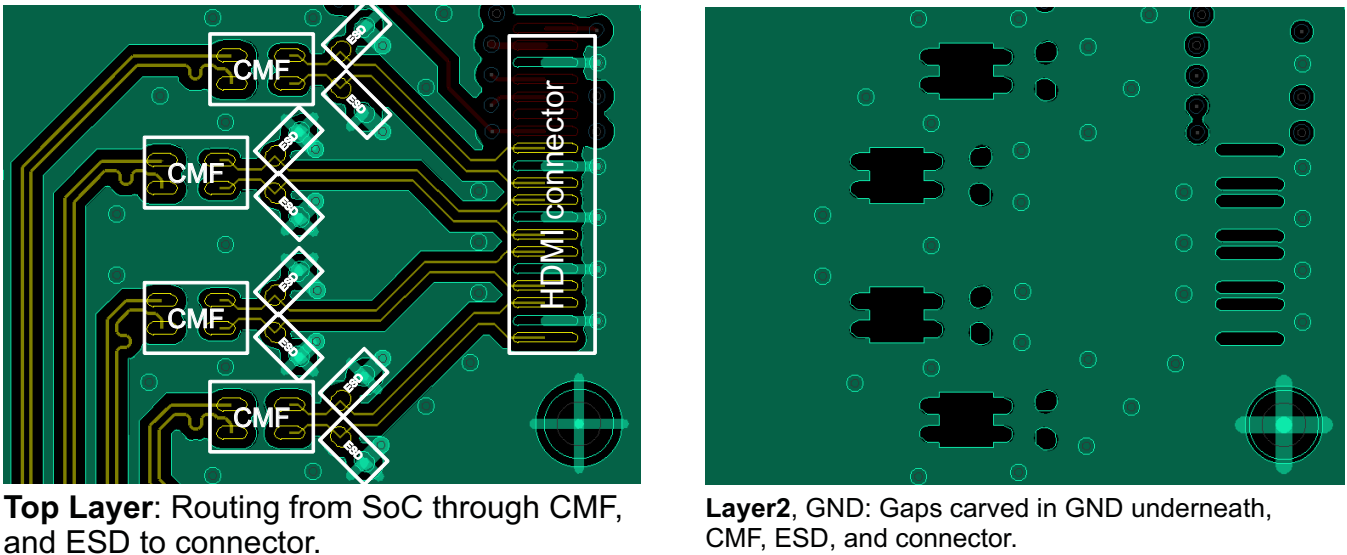
图 7-35. HDMI Example “carve GND” layout
