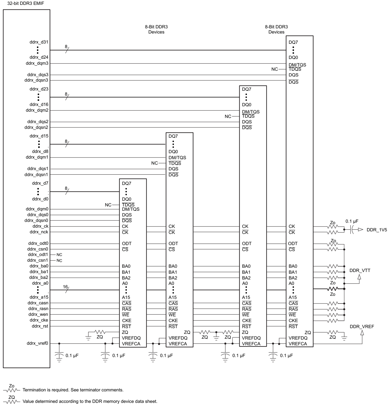
图 7-39. 32-Bit, One-Bank DDR3 Interface Schematic Using Four 8-Bit DDR3 Devices
