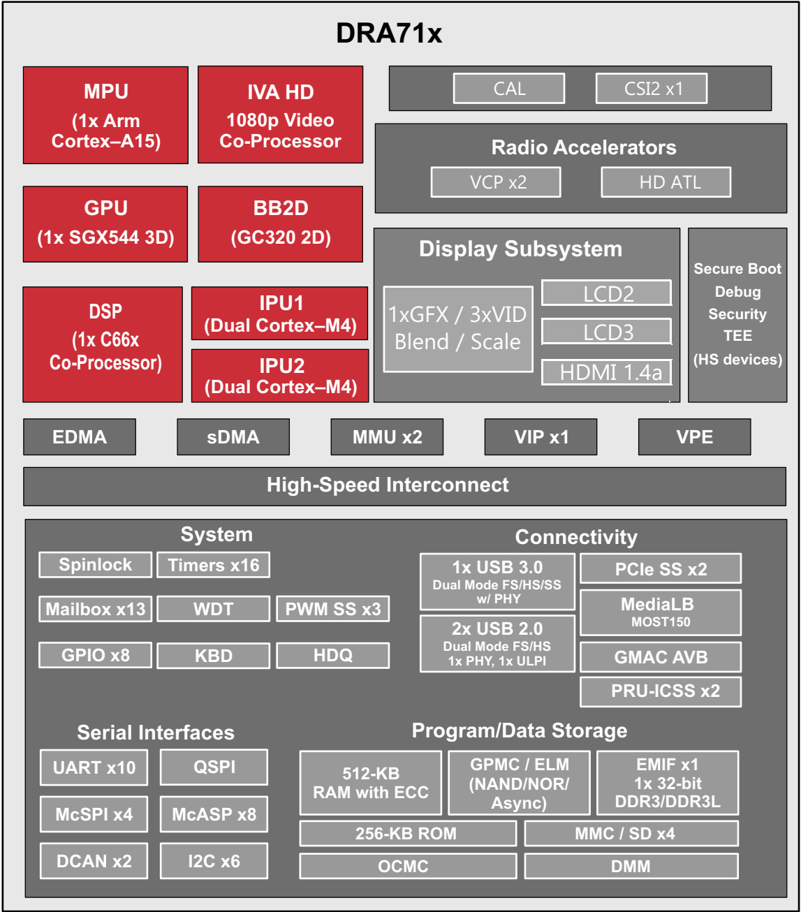
图 6-1. DRA71x Block Diagram
