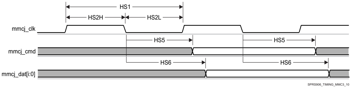
图 5-102. MMC/SD/SDIOj in - High Speed 3.3V Signaling - Transmitter Mode
