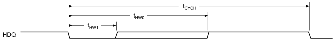
图 5-42. Device HDQ Interface Bit Read Timing (Data)
