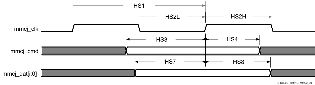
图 5-101. MMC/SD/SDIOj in - High Speed 3.3V Signaling - Receiver Mode
