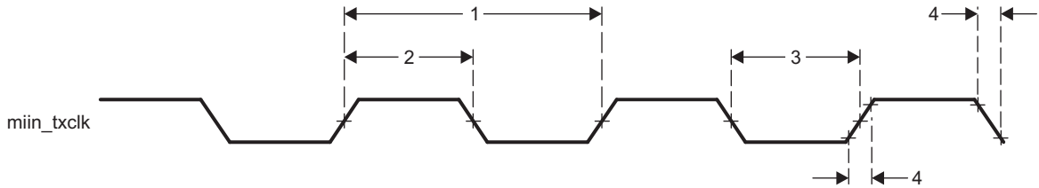
图 5-69. Clock Timing (GMAC Transmit) - MII operation
