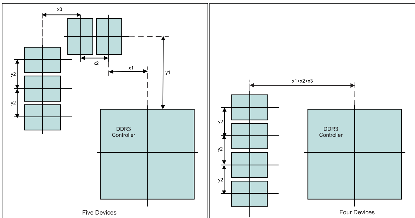
图 7-40. Placement Specifications
