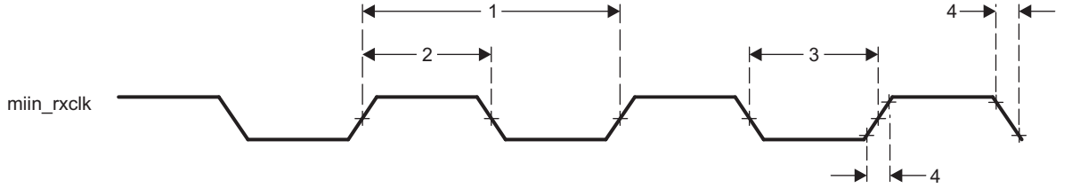
图 5-68. Clock Timing (GMAC Receive) - MII operation
