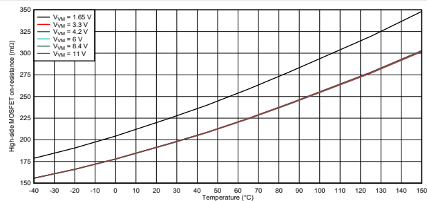
图 8-3. High-side MOSFET on resistance
