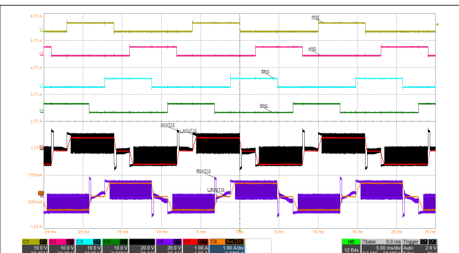
图 10-6. Stepper Motor Half-Step Operation With Fast Decay
