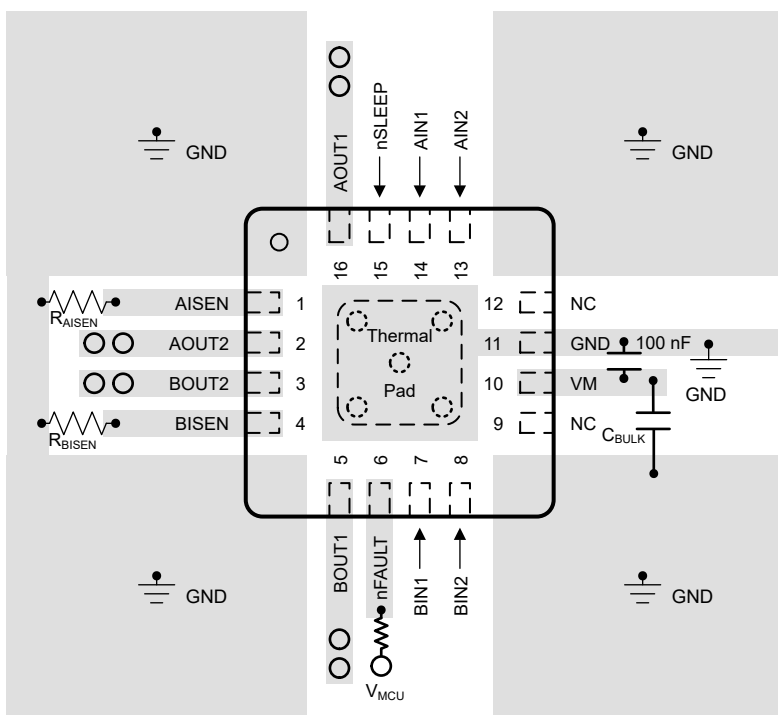
图 12-2. Recommended Layout Example for RTE (WQFN) Package
