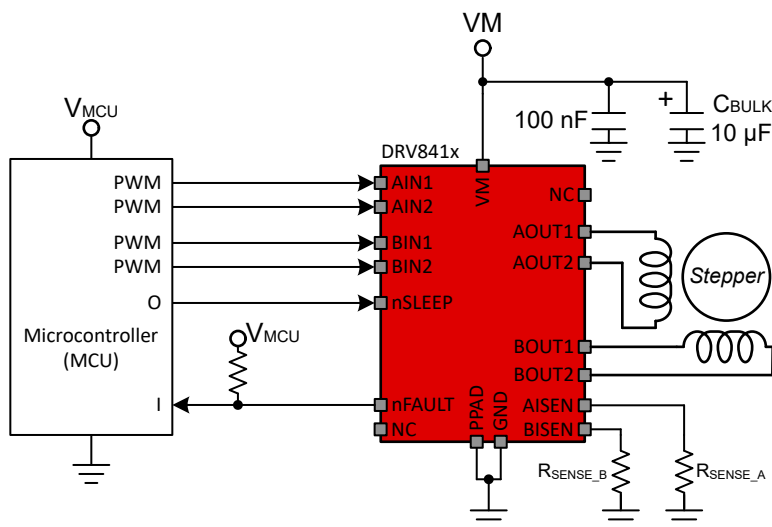
图 10-1. Typical Application Schematic of DRV8411 Driving Stepper Motor
