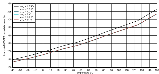
图 8-4. Low-side MOSFET on resistance
