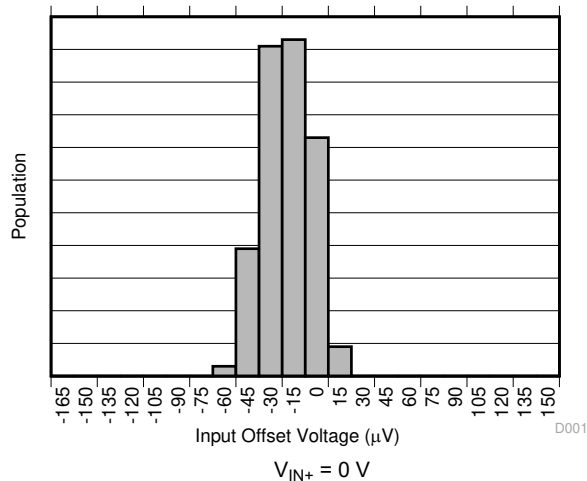
图 7-1. Input Offset Voltage Production Distribution A1
