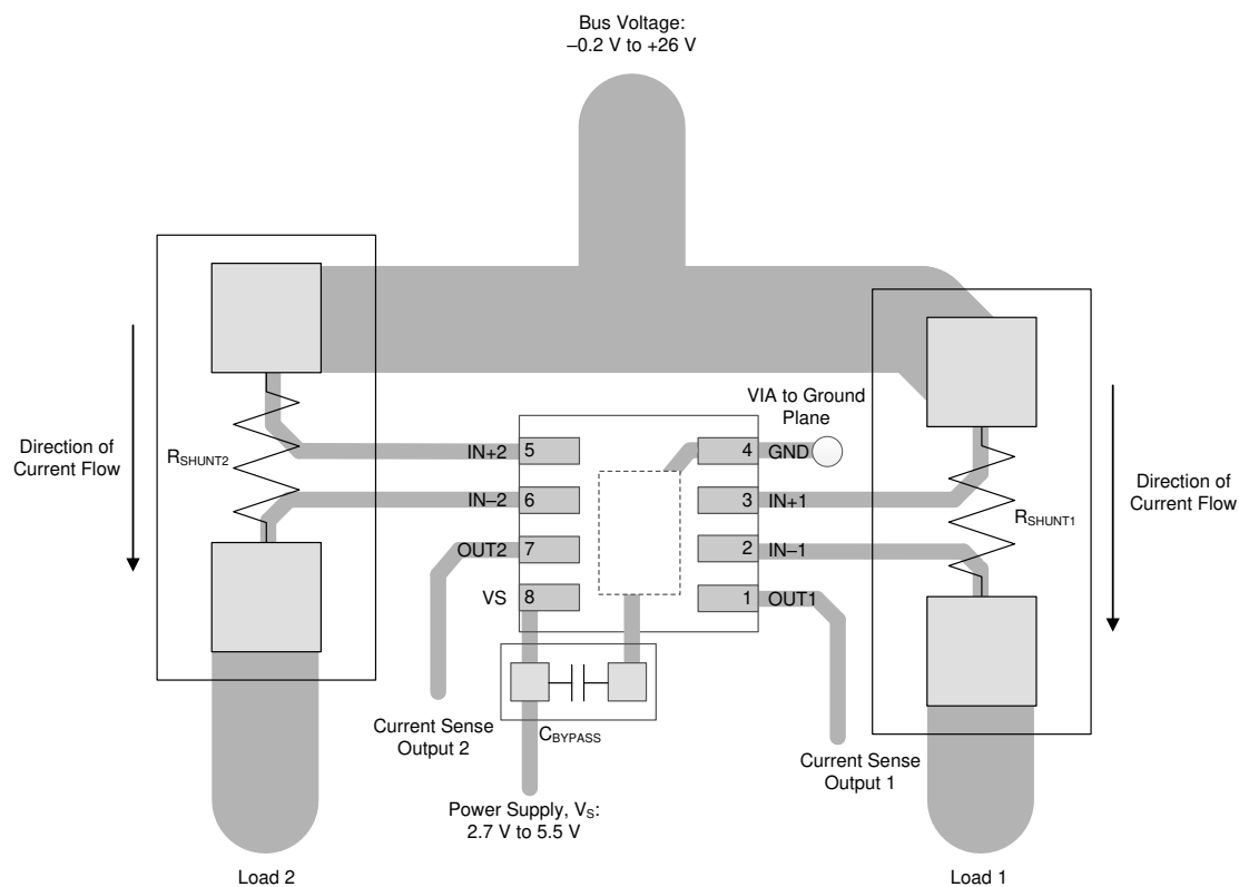
图 9-9. Dual-Channel Recommended Layout (WSO)
