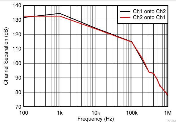
图 7-38. Channel Separation vs. Frequency (INA2180)
