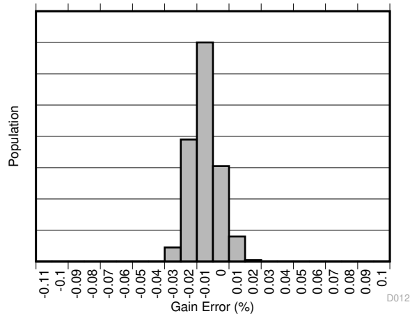
图 7-12. Gain Error Production Distribution A2
