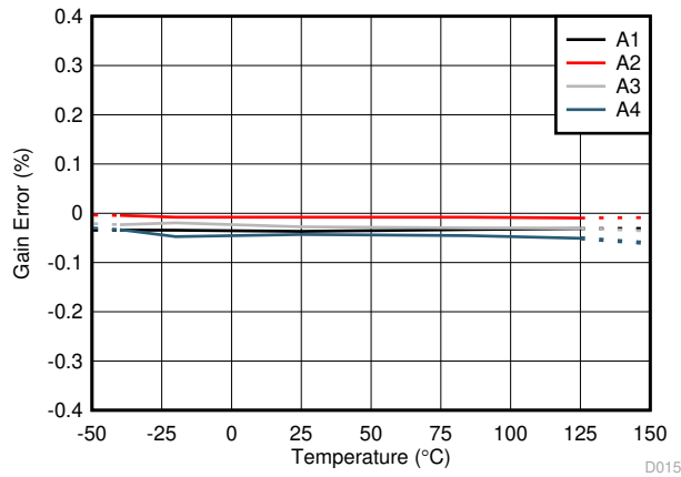
图 7-15. Gain Error vs. Temperature
