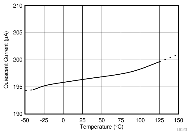
图 7-23. Quiescent Current vs. Temperature (INA180-Q1)
