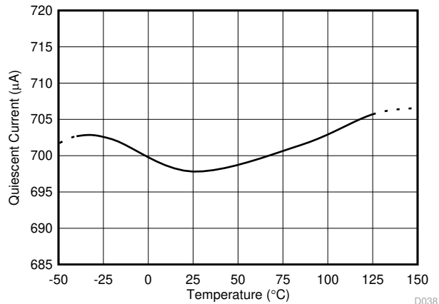
图 7-25. Quiescent Current vs. Temperature (INA4180-Q1)
