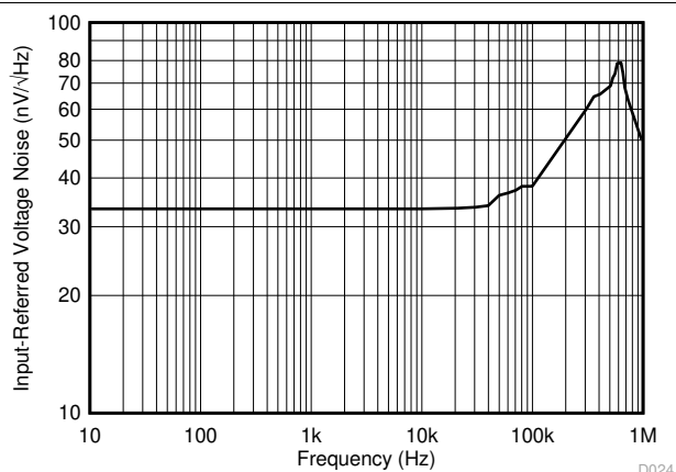
图 7-29. Input-Referred Voltage Noise vs. Frequency (A3 Devices)
