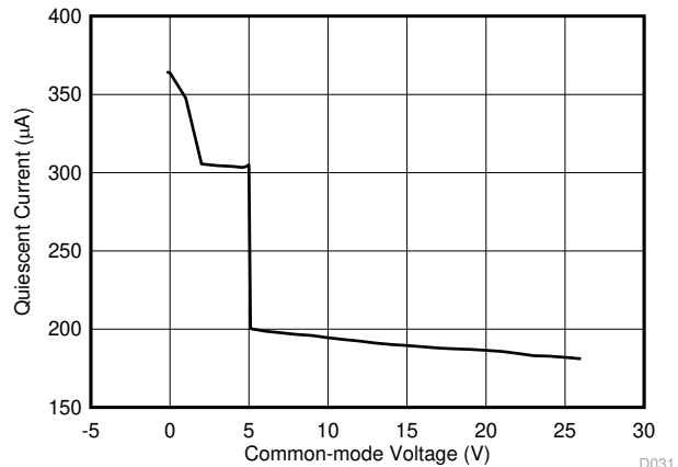
图 7-26. Quiescent Current vs. Common-Mode Voltage (INA180-Q1)
