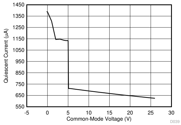
图 7-28. Quiescent Current vs. Common-Mode Voltage for All Amplifiers (INA4180-Q1)
