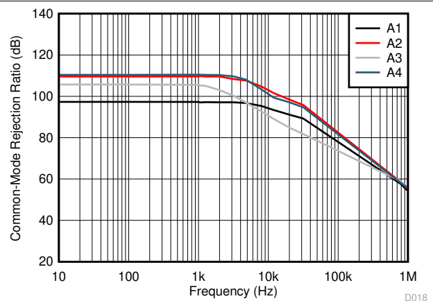
图 7-18. Common-Mode Rejection Ratio vs. Frequency
