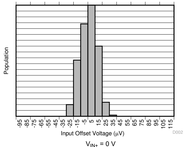
图 7-2. Input Offset Voltage Production Distribution A2
