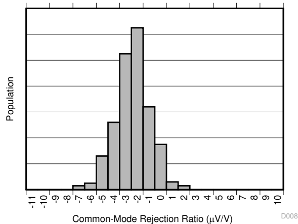
图 7-8. Common-Mode Rejection Production Distribution A3
