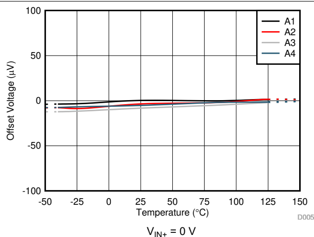
图 7-5. Offset Voltage vs. Temperature
