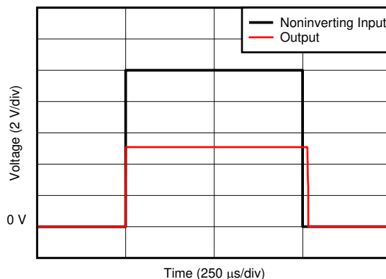
图 7-34. Noninverting Differential Input Overload
