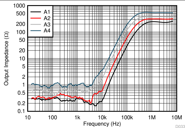
图 7-37. Output Impedance vs. Frequency
