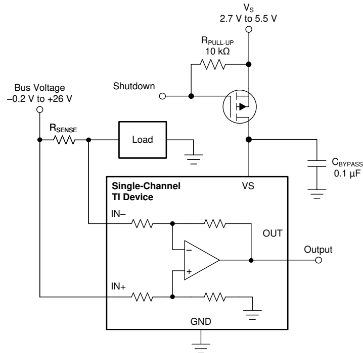
图 8-6. Basic Circuit to Shut Down the INxA180-Q1
