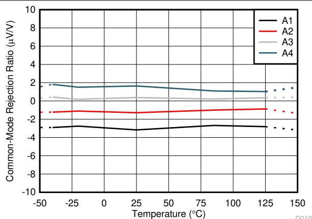
图 7-10. Common-Mode Rejection Ratio vs. Temperature
