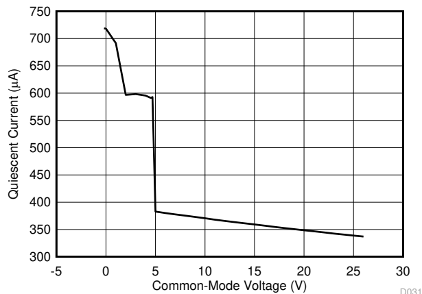
图 7-27. Quiescent Current vs. Common-Mode Voltage for All Amplifiers (INA2180-Q1)
