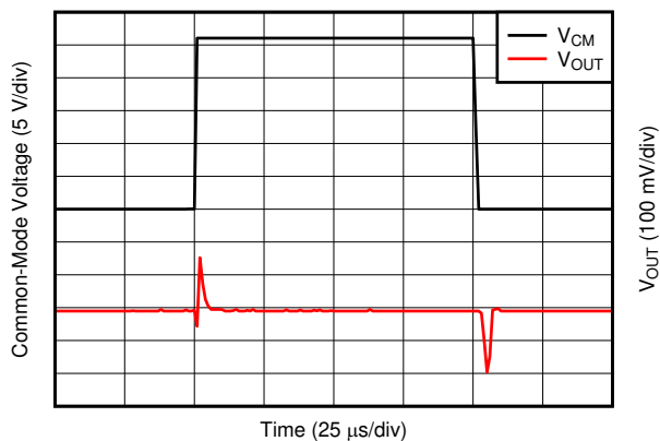
图 7-32. Common-Mode Voltage Transient Response
