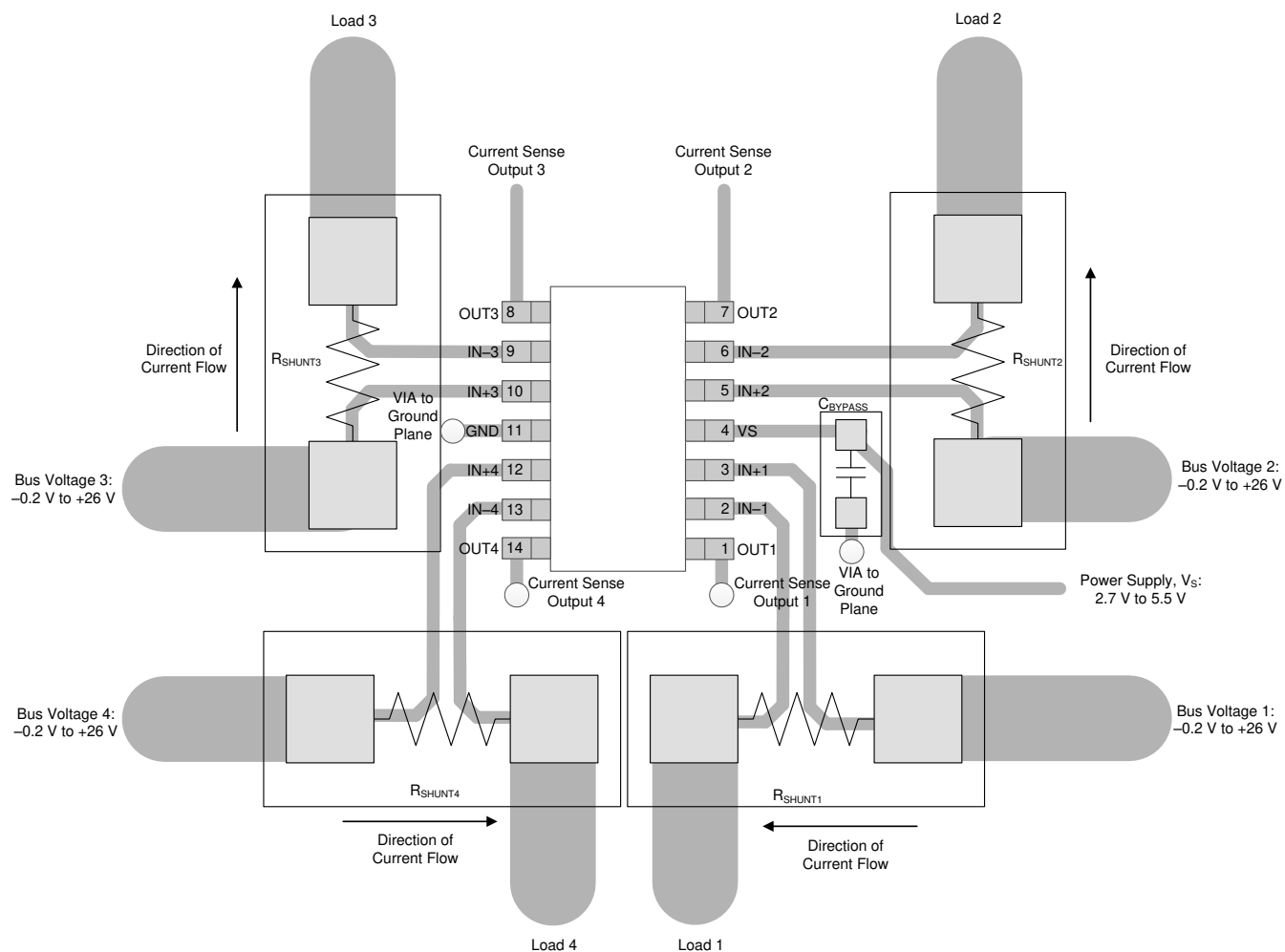
图 9-10. Quad-Channel Recommended Layout
