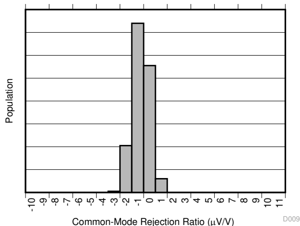
图 7-9. Common-Mode Rejection Production Distribution A4
