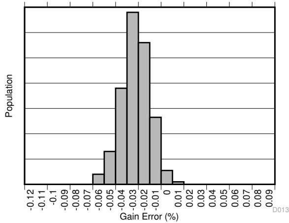
图 7-13. Gain Error Production Distribution A3
