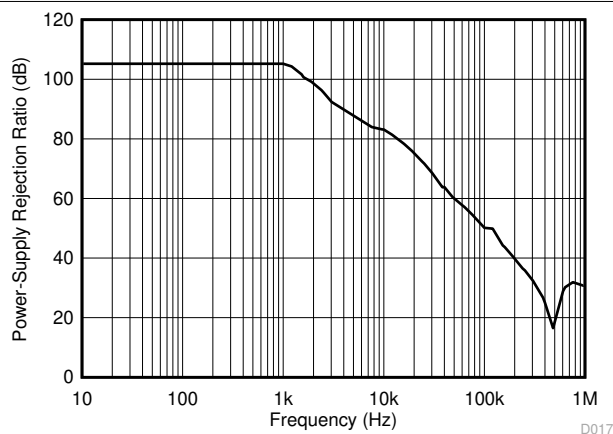
图 7-17. Power-Supply Rejection Ratio vs. Frequency
