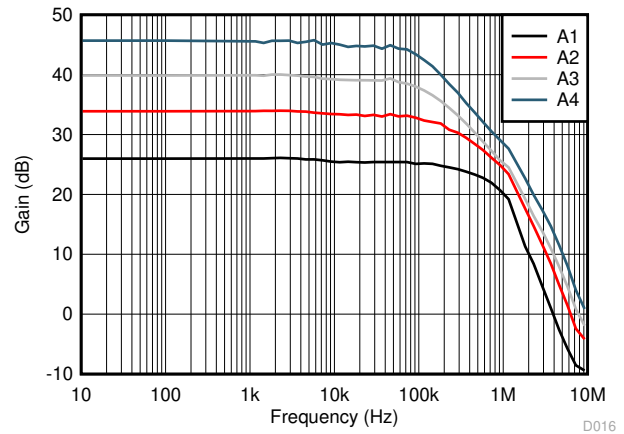
图 7-16. Gain vs. Frequency
