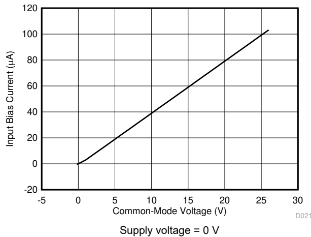
图 7-21. Input Bias Current vs. Common-Mode Voltage (Both Inputs, Shutdown)
