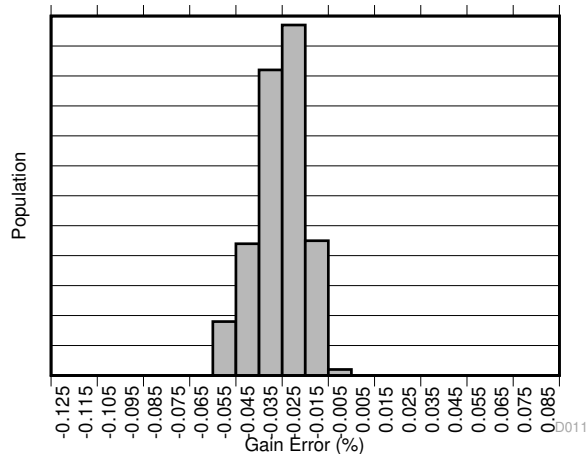
图 7-11. Gain Error Production Distribution A1
