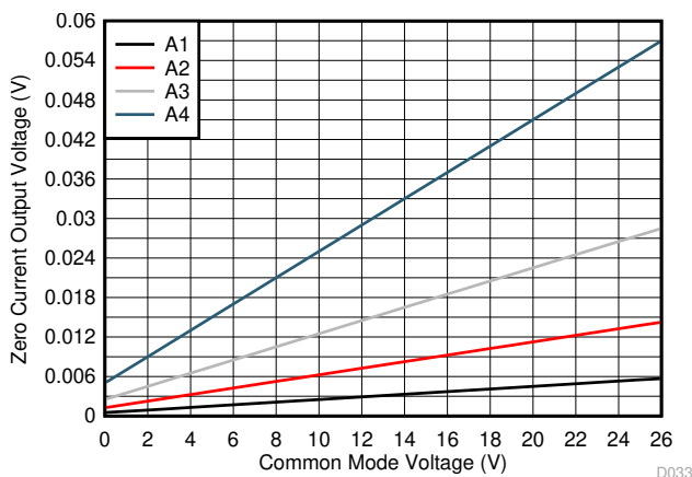
图 8-5. Zero-Current Output Voltage vs Common-Mode Voltage
