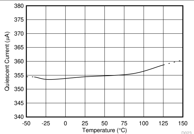
图 7-24. Quiescent Current vs. Temperature (INA2180-Q1)
