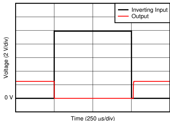
图 7-33. Inverting Differential Input Overload
