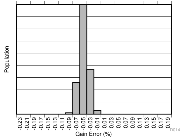
图 7-14. Gain Error Production Distribution A4
