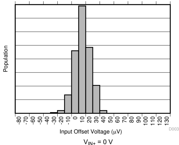
图 7-3. Input Offset Voltage Production Distribution A3
