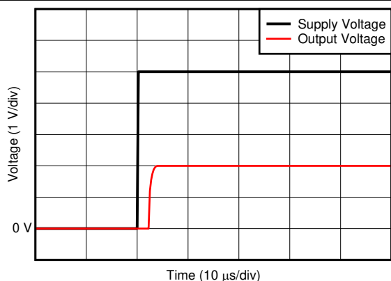
图 7-35. Start-Up Response
