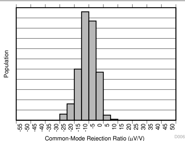
图 7-6. Common-Mode Rejection Production Distribution A1
