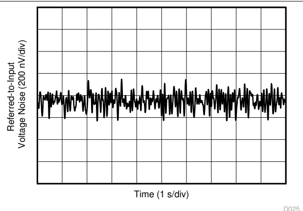
图 7-30. 0.1-Hz to 10-Hz Voltage Noise (Referred-to-Input)
