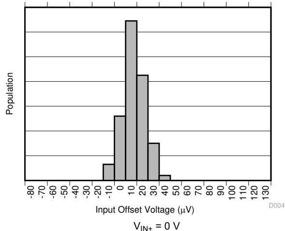
图 7-4. Input Offset Voltage Production Distribution A4
