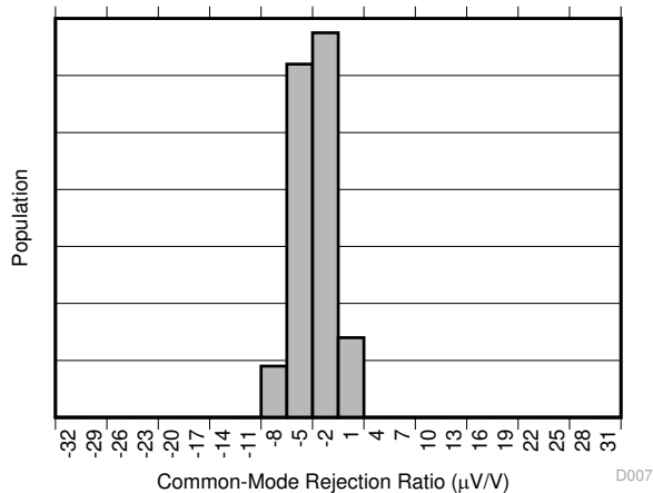
图 7-7. Common-Mode Rejection Production Distribution A2
