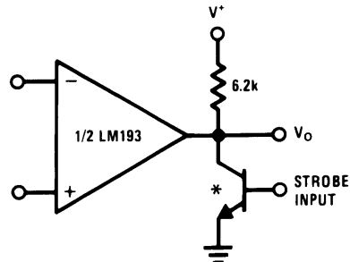
Output Strobing
