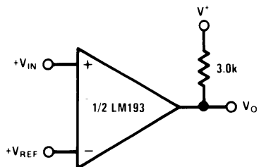
Basic Comparator
