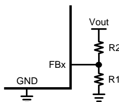
Figure 31. Output Voltage Setting
