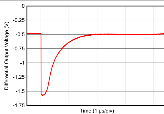
图 6-20. Ambient Loop Cancellation Settling Time (1)
