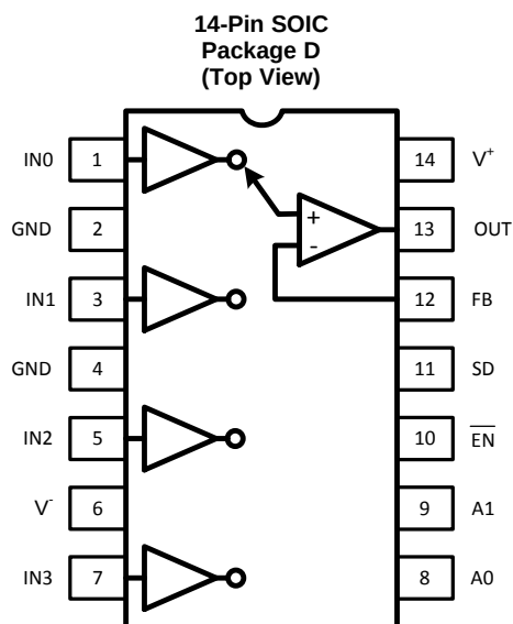
Pin Functions
