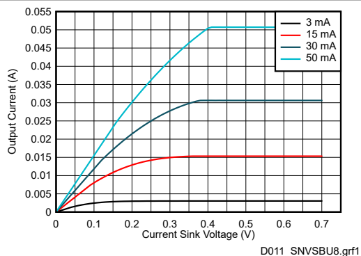
图 7-9. Current Sinks Voltage vs Current
