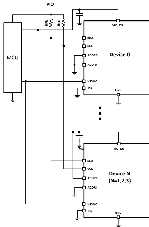
图 8-13. I²C Multiple Devices Connection
