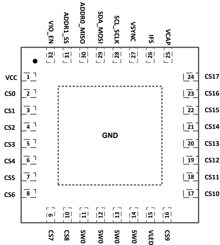
图 6-1. LP5861 RSM Package 32-Pin VQFN with Exposed Thermal Pad Top View
