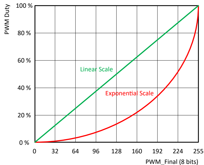
图 8-2. Linear and Exponential Dimming Curves
