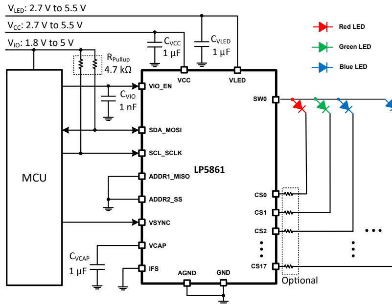
图 9-1. Typical Application - LP5861 Driving 6 RGB LEDs
