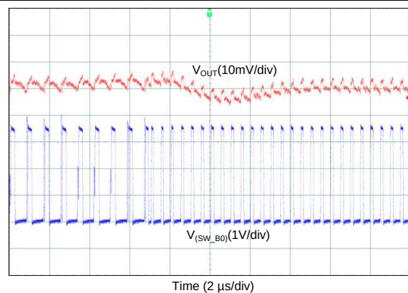
图 86. Transient from PFM-to-PWM Mode (3-Phase Output)
