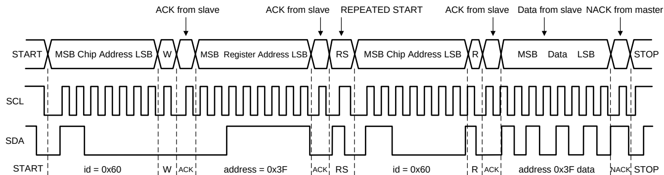
图 26. Read Cycle ( r = \text{read} ; \text{SDA} = 1 ), Using Example \text{id} = \text{Device Address} = 0x60 for LP8756x-Q1
