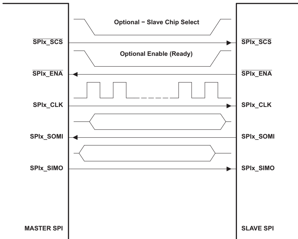
Figure 5-38. Illustration of SPI Master-to-SPI Slave Connection
