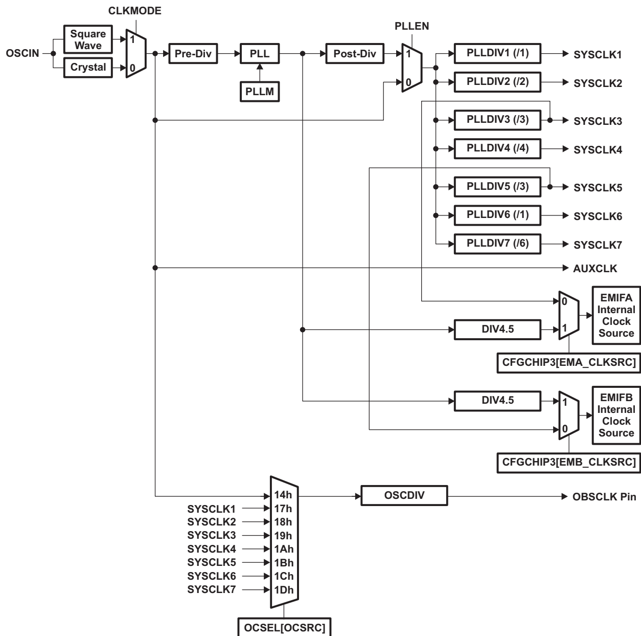
Figure 5-10. PLL Topology
