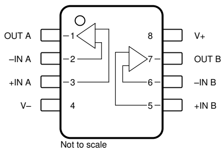
图 5-2. OPA2205 DGK (8-Pin VSSOP) Package, Top View
