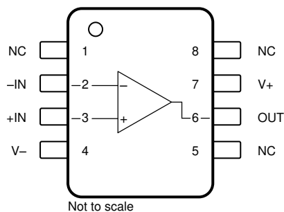
图 5-1. OPA205 D (8-Pin SOIC) PREVIEW Package, Top View
