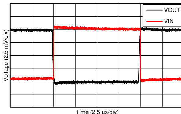
图 6-28. Negative Overload Recovery
