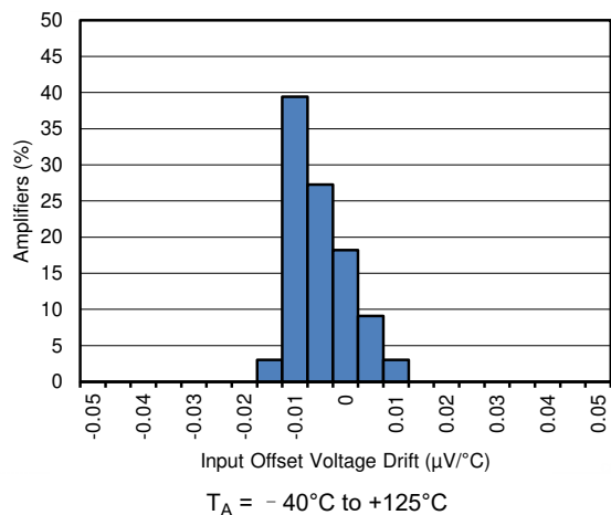
图 6-2. Offset Voltage Drift Distribution
