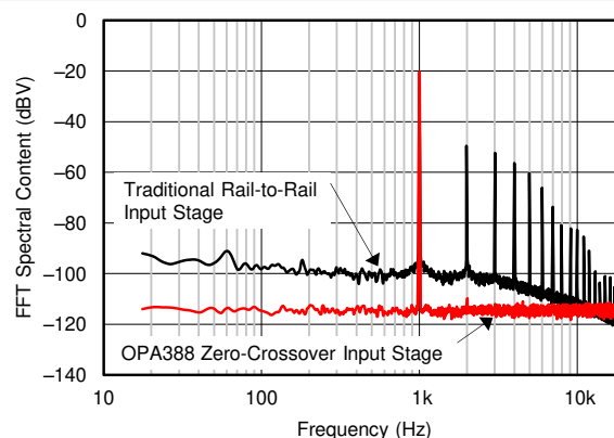
图 7-2. Input Crossover Distortion Spectral Content
