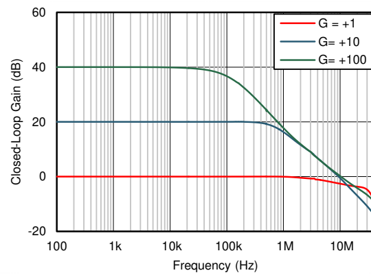
图 6-8. Closed-Loop Gain and Phase vs Frequency
