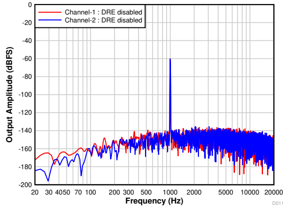
图 7-11. PCM1820: FFT With a -60-dBr Input and DRE Disabled
