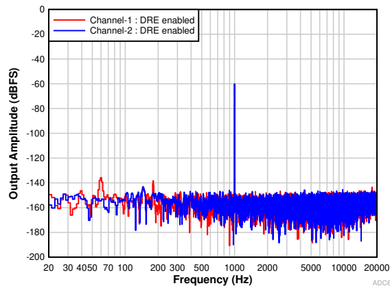
图 9-2. PCM1820: FFT With a -60-dBr Input With DRE Enabled
