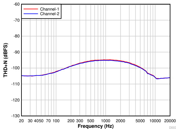
图 7-15. PCM1821: THD+N vs Input Frequency With a -1-dBr Input
