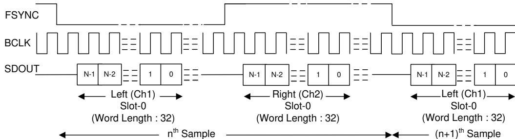
图 8-3. I 2 S Mode Protocol Timing (FMT0 = LOW) in Slave Mode
