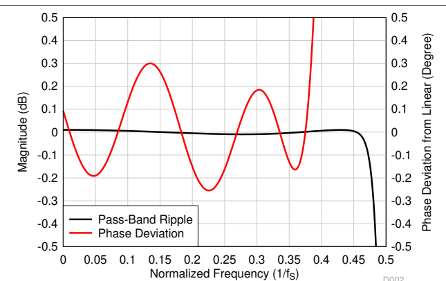
图 8-24. Low-Latency Decimation Filter Pass-Band Ripple and Phase Deviation
