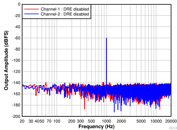
图 9-4. PCM1820: FFT With a -60-dBr Input With DRE Disabled
