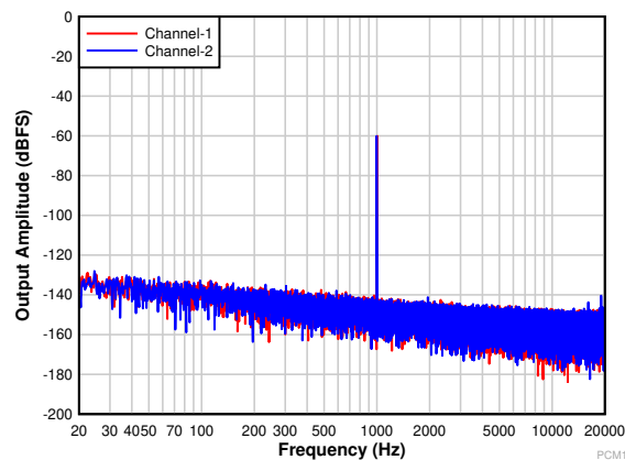
图 9-6. PCM1821: FFT With a -60-dBr Input
