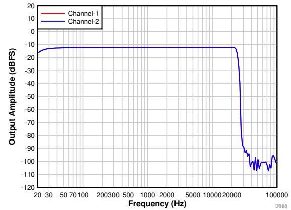
图 7-6. PCM1820: Frequency Response With a -12\text{-dBr} Input
