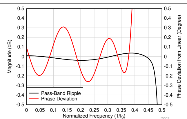
图 8-26. Low-Latency Decimation Filter Pass-Band Ripple and Phase Deviation
