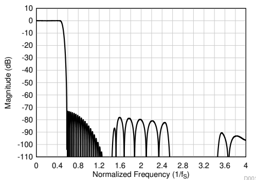
图 8-11. Linear Phase Decimation Filter Magnitude Response
