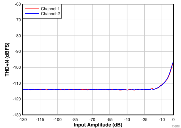
图 7-2. PCM1820: THD+N vs Input Amplitude With DRE Disabled
