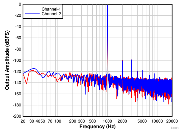
图 7-20. PCM1821: FFT With a -1-dBr Input
