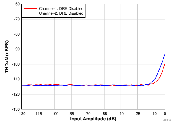
图 9-5. PCM1820: THD+N vs Input Amplitude With DRE Disabled
