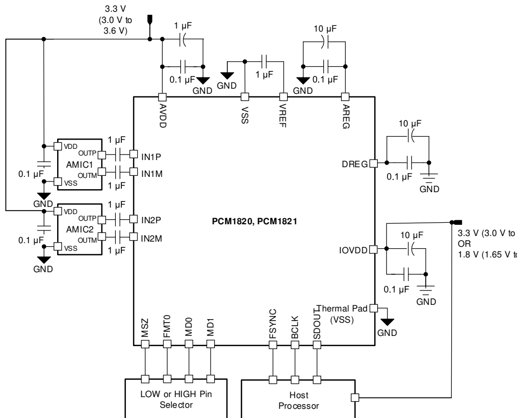
图 9-1. Two-Channel Analog Microphone Recording Diagram for 3.3-V AVDD Operation
