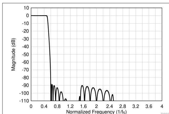
图 8-25. Low-Latency Decimation Filter Magnitude Response
