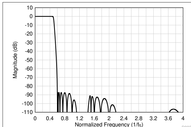
图 8-23. Low-Latency Decimation Filter Magnitude Response
