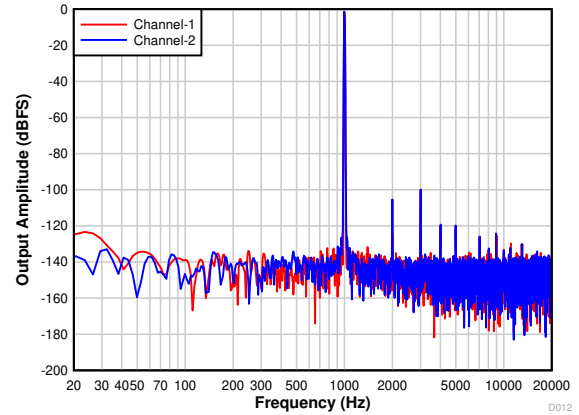
图 7-12. PCM1820: FFT With a -1-dBr Input
