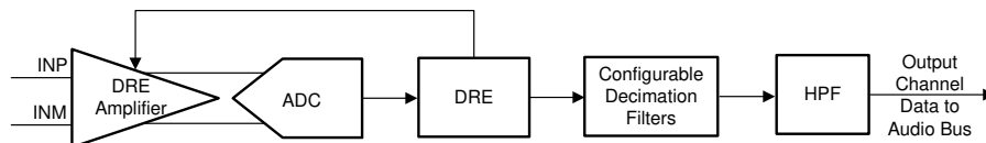
图 8-5. Signal-Chain Processing Flowchart
