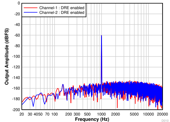
图 7-10. PCM1820: FFT With a -60\text{-dBr} Input and DRE Enabled
