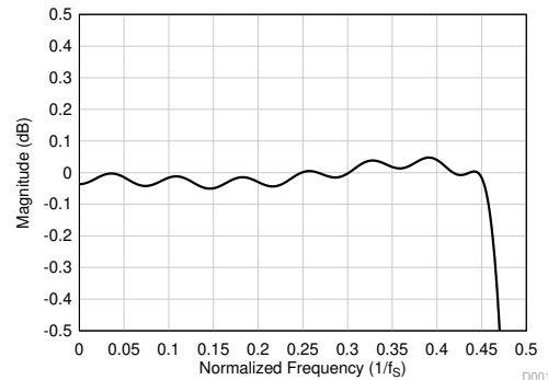
图 8-14. Linear Phase Decimation Filter Pass-Band Ripple
