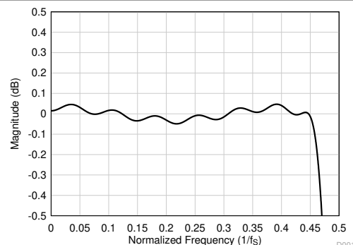
图 8-16. Linear Phase Decimation Filter Pass-Band Ripple
