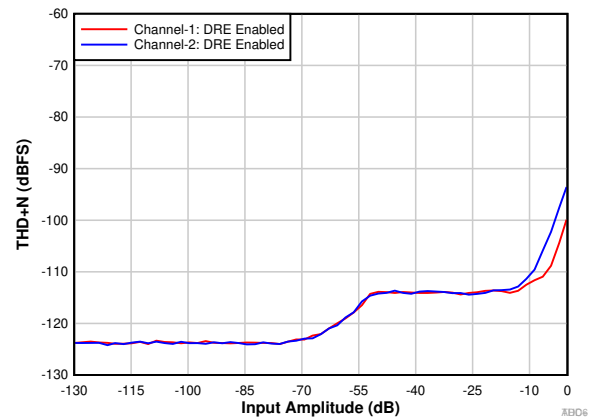
图 9-3. PCM1820: THD+N vs Input Amplitude With DRE Enabled
