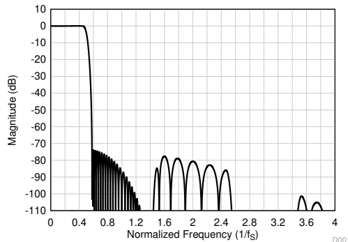
图 8-13. Linear Phase Decimation Filter Magnitude Response
