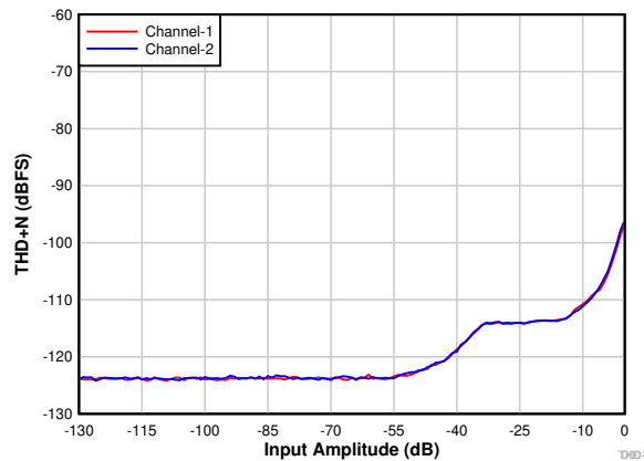
图 7-1. PCM1820: THD+N vs Input Amplitude With DRE Enabled
