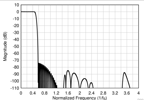
图 8-15. Linear Phase Decimation Filter Magnitude Response
