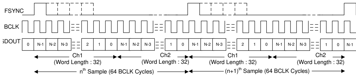
图 8-2. TDM Mode Protocol Timing (FMT0 = HIGH) In Master Mode
