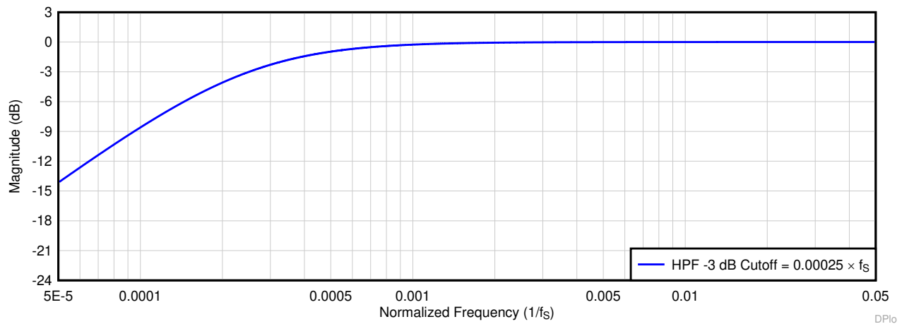
图 8-6. HPF Filter Frequency Response Plot
