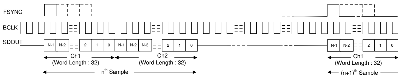
图 8-1. TDM Mode Protocol Timing (FMT0 = HIGH) In Slave Mode
