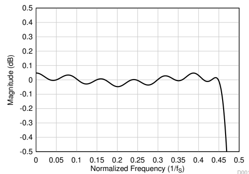
图 8-12. Linear Phase Decimation Filter Pass-Band Ripple
