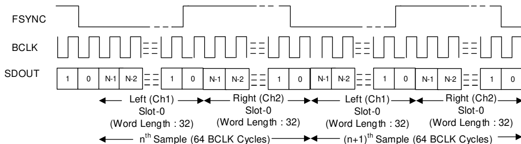
图 8-4. I 2 S Protocol Timing (FMT0 = LOW) In Master Mode
