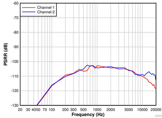
图 7-17. PCM1821: Power-Supply Rejection Ratio vs Ripple Frequency With a 100-mV PP Amplitude
