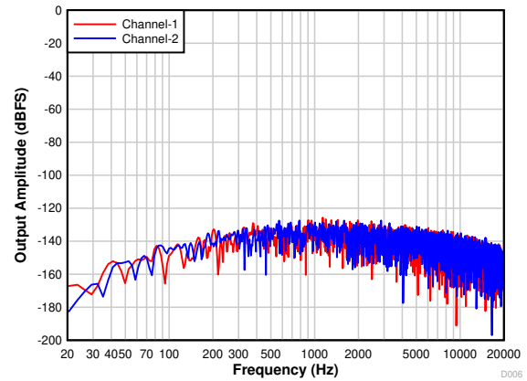
图 7-18. PCM1821: FFT With Idle Input
