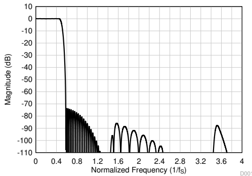
图 8-17. Linear Phase Decimation Filter Magnitude Response
