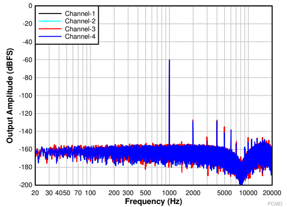
图 8-2. FFT With a -60-dBr Input
