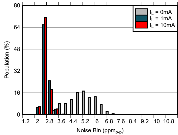
图 7-10. 0.1 Hz to 10 Hz Noise Distribution ( V_{REF} = 2.5\text{ V} , C_L = 1\text{ }\mu\text{F} , C_{NR} = \text{Open} )
