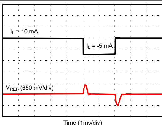
图 7-21. Load Transient Response ( V_{REF} = 1.25\text{ V} , C_L = 1\text{ }\mu\text{F} )
