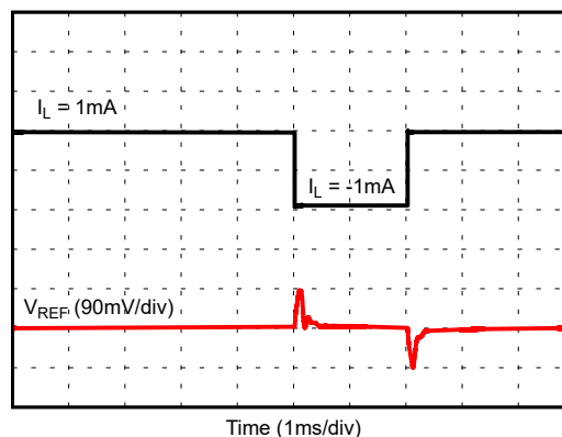
图 7-20. Load Transient Response ( V_{REF} = 1.25\text{ V} , C_L = 1\text{ }\mu\text{F} )
