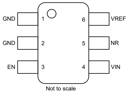
图 6-1. DBV Package 6-Pin SOT-23 Top View
