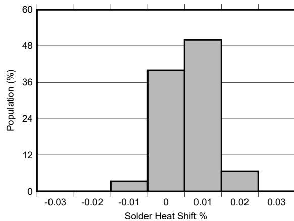
图 7-29. Solder Heat Shift Distribution
