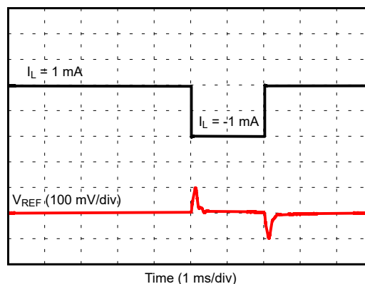
图 7-18. Load Transient Response ( V_{REF} = 2.5\text{ V} , C_L = 1\text{ }\mu\text{F} )
