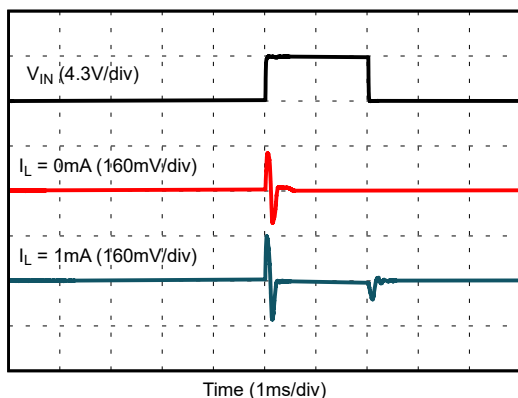
图 7-23. Line Transient Response ( V_{REF} = 1.25\text{ V} , C_L = 1\text{ }\mu\text{F} )
