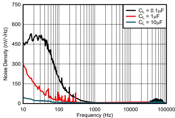
图 7-11. Noise Density vs Frequency ( V_{REF} = 1.25\text{ V} , I_L = 0\text{ mA} )
