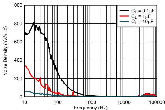
图 8-15. Noise Spectrum 10 Hz to 100 kHz ( V_{REF} = 2.5\text{ V} )
