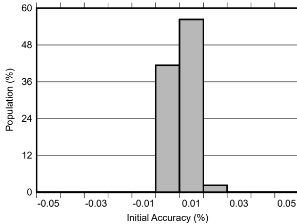
图 7-5. Initial Accuracy Distribution
