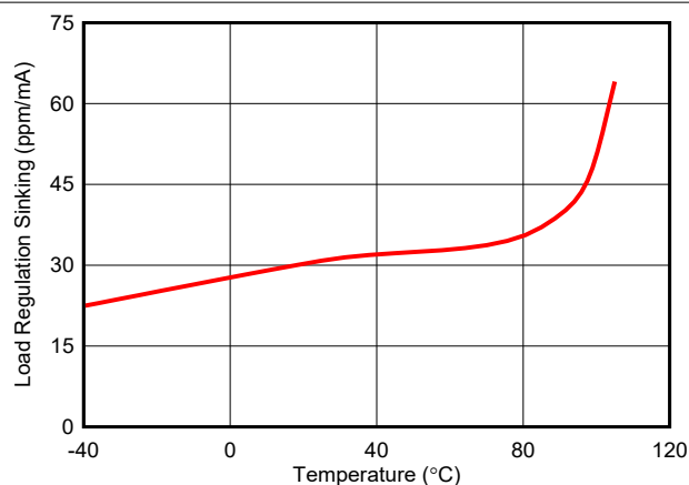
图 7-15. Load Regulation (Sinking 5 mA) vs Free-Air Temperature
