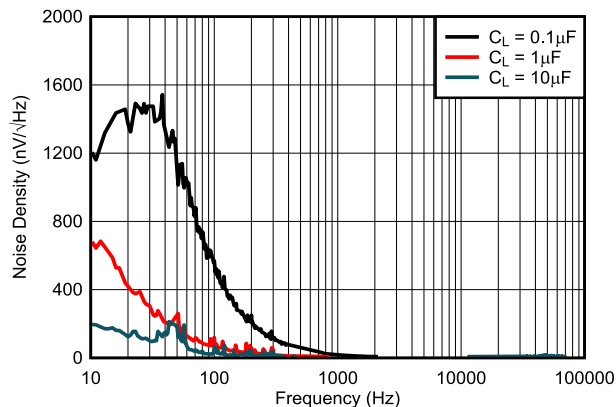
图 7-13. Noise Density vs Frequency ( V_{REF} = 5\text{ V} , I_L = 0\text{ mA} )
