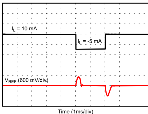
图 7-19. Load Transient Response ( V_{REF} = 2.5\text{ V} , C_L = 1\text{ }\mu\text{F} )
