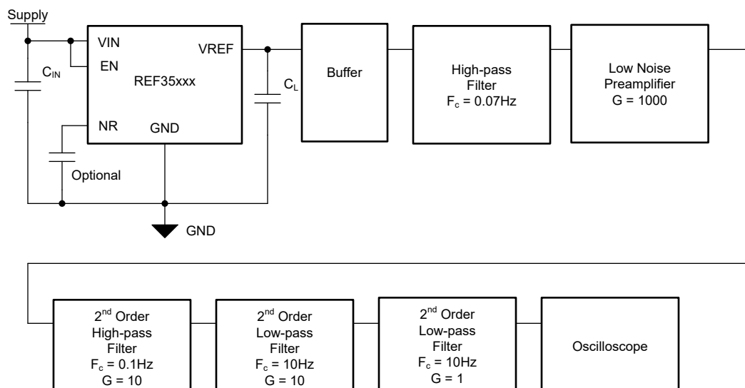
图 8-10. Low-Frequency (1/f) Noise Test Setup
