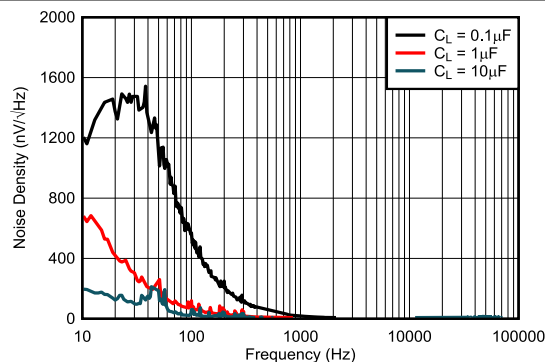
图 8-16. Noise Spectrum 10 Hz to 100 kHz ( V_{REF} = 5\text{ V} )
