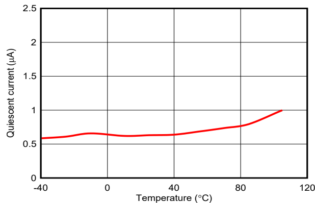
图 7-27. Quiescent Current vs Free-Air Temperature
