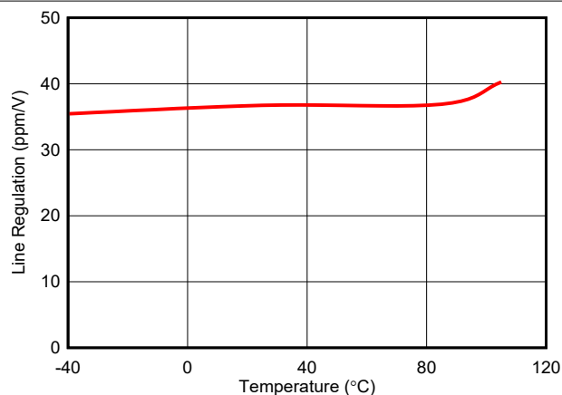
图 7-22. Line Regulation vs Free-Air Temperature
