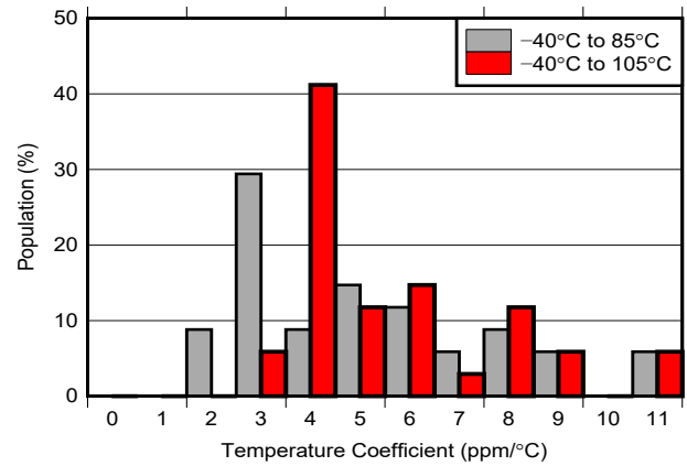
图 7-4. Temperature Coefficient Distribution ( V_{REF} = 5.0\text{ V} )
