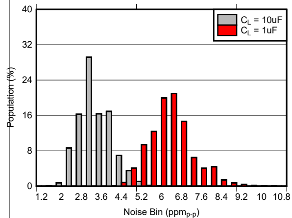
图 7-6. 0.1 Hz to 10 Hz Noise Distribution ( V_{REF} = 1.25\text{ V} , C_{NR} = \text{Open} , I_L = 0\text{ mA} )
