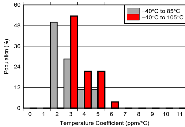
图 7-3. Temperature Coefficient Distribution ( V_{REF} = 2.5\text{ V} )
