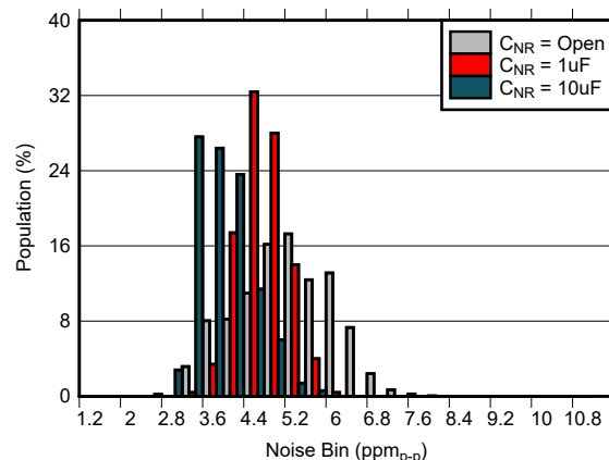
图 8-13. 0.1 Hz to 10 Hz Noise Distribution vs NR Capacitance
