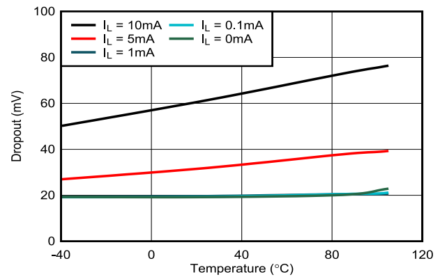
图 7-28. Dropout Voltage vs Free-Air Temperature
