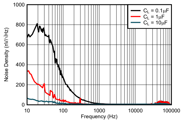
图 7-12. Noise Density vs Frequency ( V_{REF} = 2.5\text{ V} , I_L = 0\text{ mA} )
