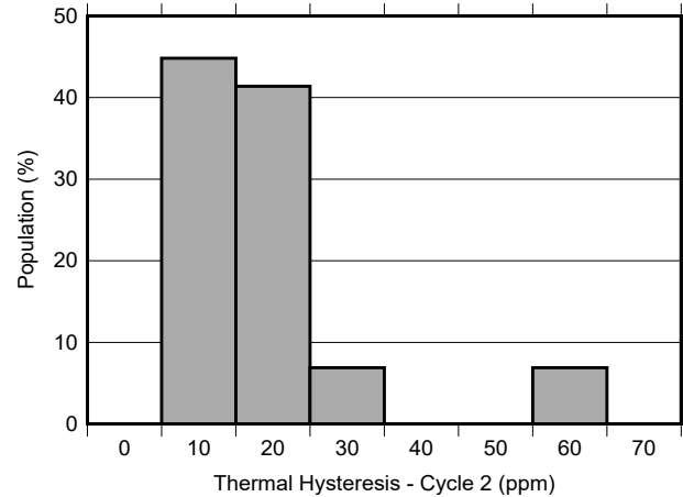
图 8-7. Thermal Hysteresis Distribution - 40°C to 85°C, Cycle 2
