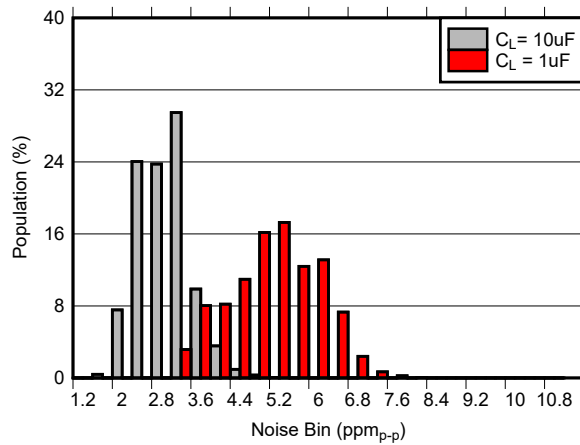
图 7-7. 0.1 Hz to 10 Hz Noise Distribution ( V_{REF} = 2.5\text{ V} , C_{NR} = \text{Open} , I_L = 0\text{ mA} )
