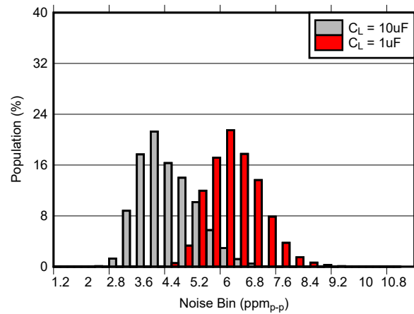
图 7-8. 0.1 Hz to 10 Hz Noise Distribution ( V_{REF} = 5\text{ V} , C_{NR} = \text{Open} , I_L = 0\text{ mA} )
