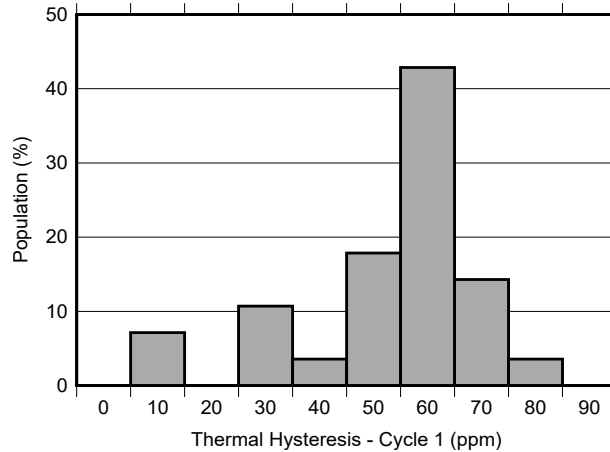
图 8-6. Thermal Hysteresis Distribution - 40°C to 85°C, Cycle 1
