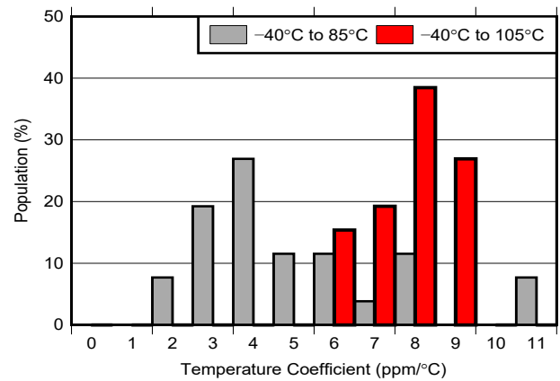
图 7-2. Temperature Coefficient Distribution ( V_{REF} = 1.25\text{ V} )
