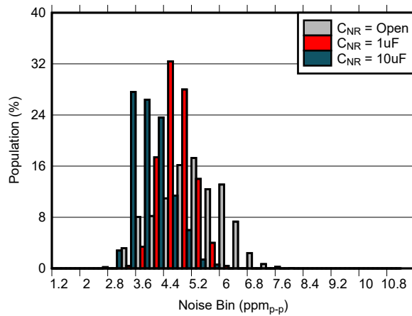
图 7-9. 0.1 Hz to 10 Hz Noise Distribution ( V_{REF} = 2.5\text{ V} , C_L = 1\text{ }\mu\text{F} , I_L = 0\text{ mA} )
