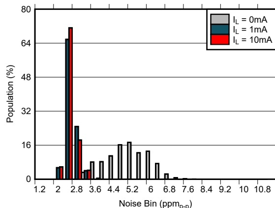
图 8-12. 0.1 Hz to 10 Hz Noise Distribution vs Load Conditions
