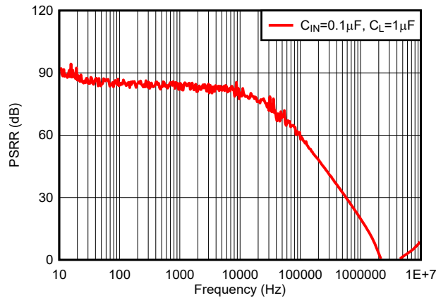
图 7-25. Power Supply Rejection Ratio ( V_{REF} = 2.5\text{ V} , I_L = 0\text{ mA} )
