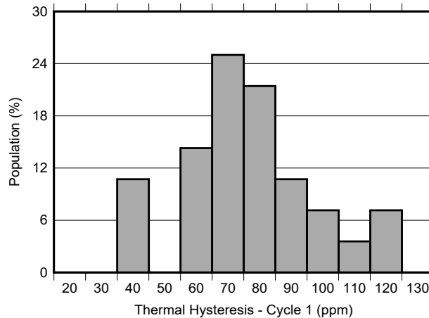
图 8-8. Thermal Hysteresis Distribution - 40°C to 105°C, Cycle 1
