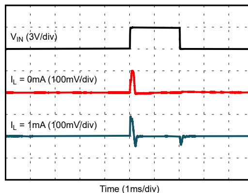
图 7-24. Line Transient Response ( V_{REF} = 2.5\text{ V} , C_L = 1\text{ }\mu\text{F} )
