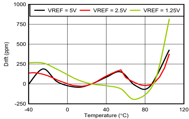
图 7-1. Output Voltage Drift vs Free-Air Temperature
