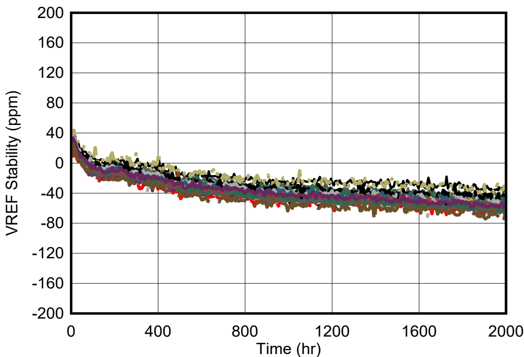
图 8-5. Long Term Stability - 2000 hours ( V_{REF} )
