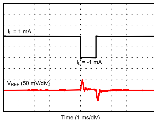
图 7-16. Load Transient Response ( V_{REF} = 2.5\text{ V} , C_L = 10\text{ }\mu\text{F} )
