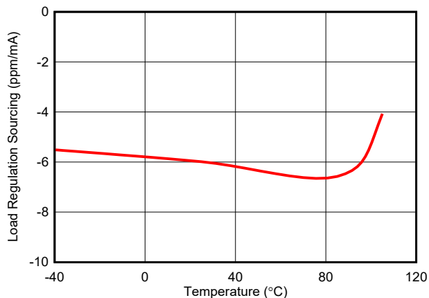
图 7-14. Load Regulation (Sourcing 10 mA) vs Free-Air Temperature
