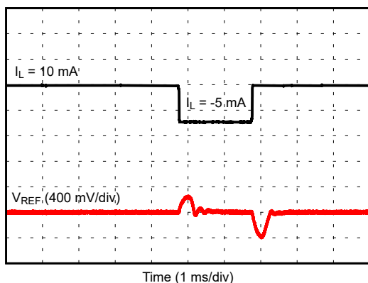
图 7-17. Load Transient Response ( V_{REF} = 2.5\text{ V} , C_L = 10\text{ }\mu\text{F} )
