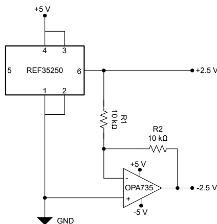
图 10-1. REF35 and OPA735 Create Positive and Negative Reference Voltages
