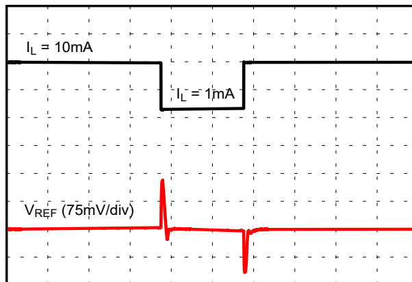
图 9-4. Load Transient Response 1 mA to 10 mA, C_L = 1 \mu F
