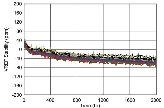
图 7-30. Long Term Stability - 2000 hours ( V_{REF} )
