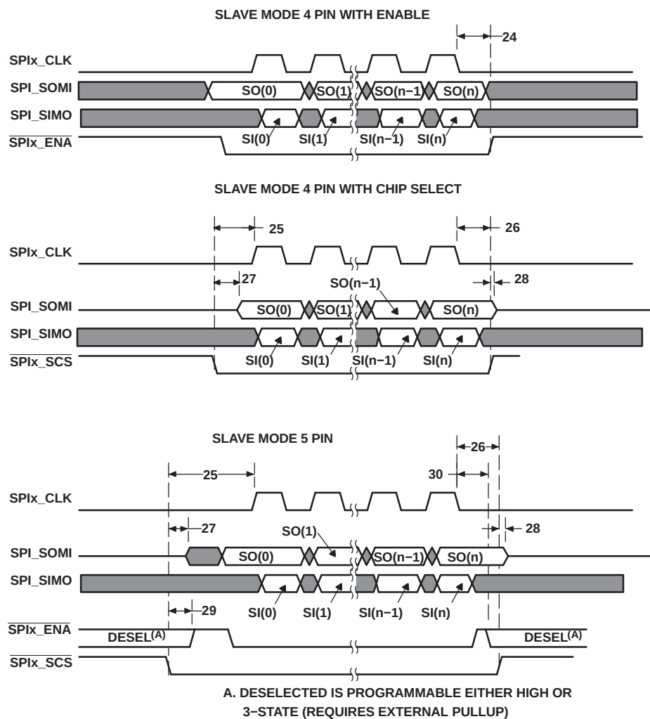
Figure 4-38. SPI Timings—Slave Mode (4-Pin and 5-Pin)
