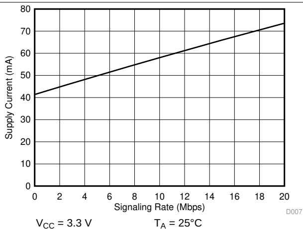
图 12. SN65HVD73, SN65HVD74 Supply Current vs Signal Rate
