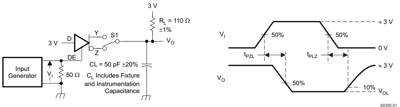
图 19. Measurement of Driver Enable and Disable Times with Active-Low Output and Pullup Load
