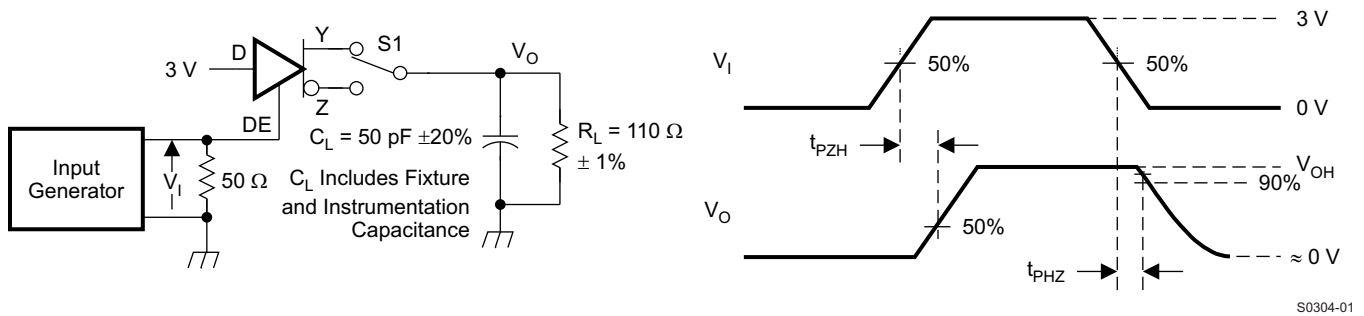
图 18. Measurement of Driver Enable and Disable Times with Active-High Output and Pulldown Load
