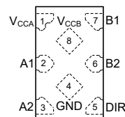
图 5-4. DTM Package, 8-Pin X2SON Transparent (Top View)
