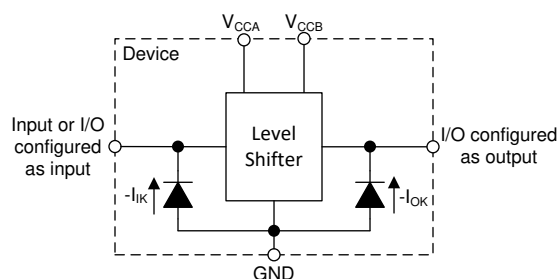
图 13-1. Electrical Placement of Clamping Diodes for Each Input and Output
