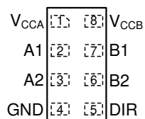
图 5-3. DTT Package, 8-Pin SON Transparent (Top View)
