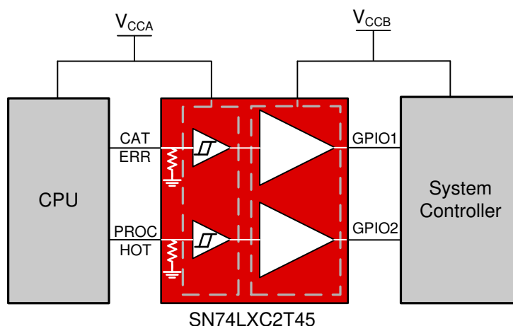
图 17-1. GPIO Driver Application
