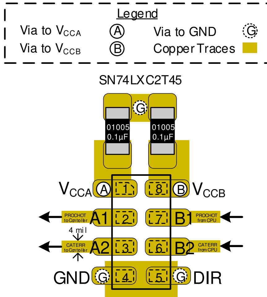
图 19-1. Layout Example—SN74LXC2T45DTT
