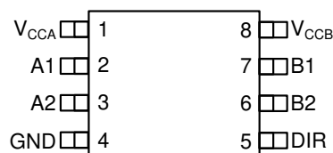
图 5-2. DCU Package, 8-Pin VSSOP (Top View)
