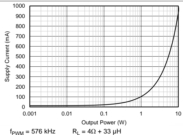
图 53. Supply Current vs. Output Power
