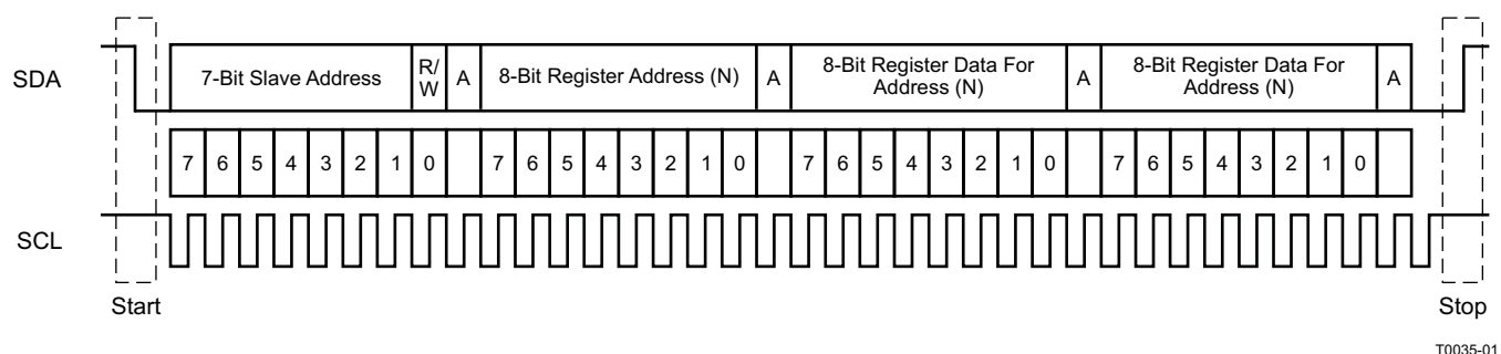
图 28. Typical I 2 C Timing Sequence
