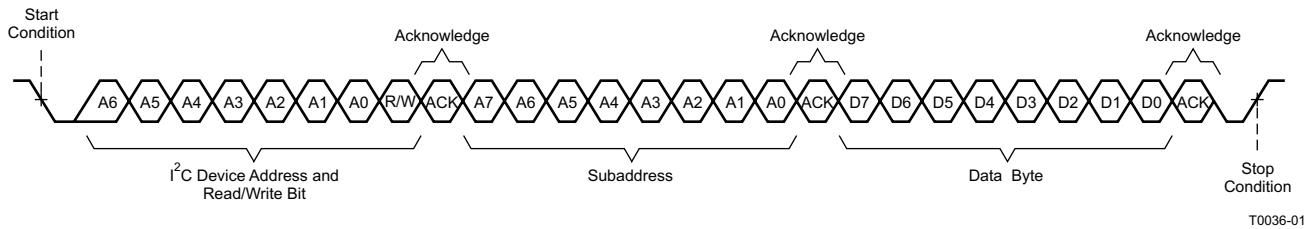
图 61. Single-Byte Write Transfer
