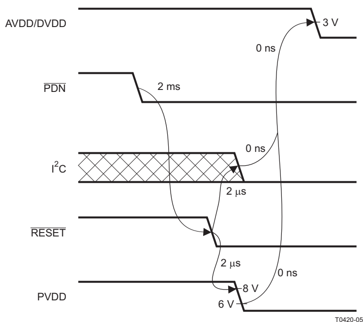
图 70. Power-Loss Sequence
