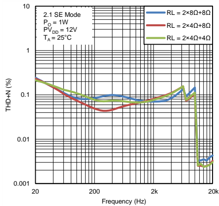
图 9. Total Harmonic Distortion + Noise vs Frequency
