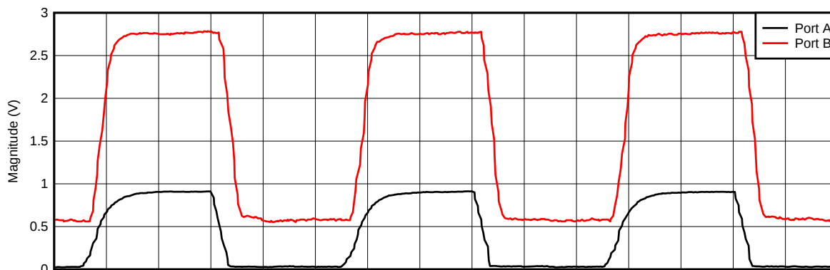
Figure 12. Voltage Translation at 400 kHz, V_{CCA} = 0.9 V, V_{CCB} = 2.7 V
