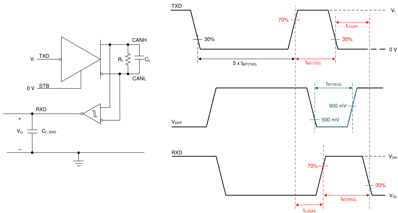
图 8-4. Transmitter and Receiver Timing Test Circuit and Measurement
