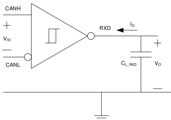
图 7-3. Receiver Test Circuit and Measurement
