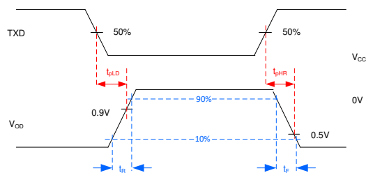
图 7-2. Driver Test Circuit and Measurement
