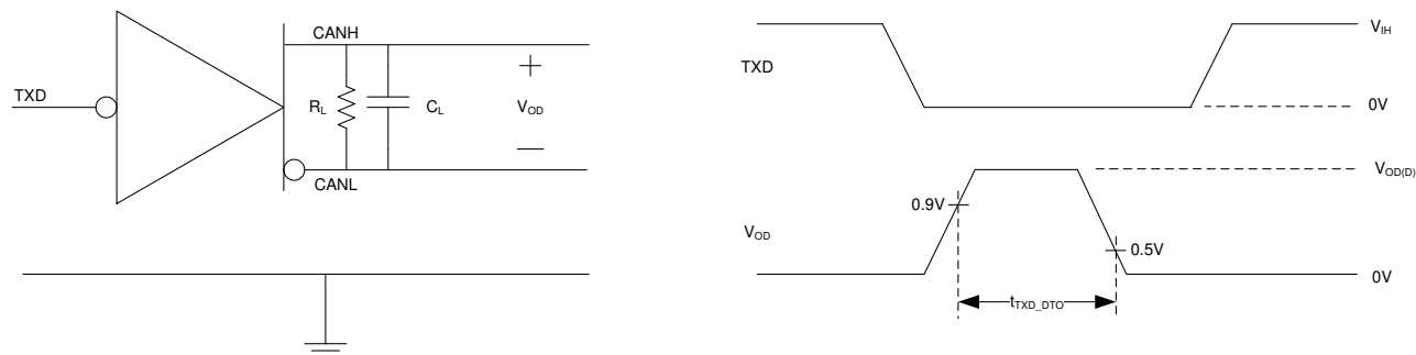
图 7-6. TXD Dominant Timeout Test Circuit and Measurement
