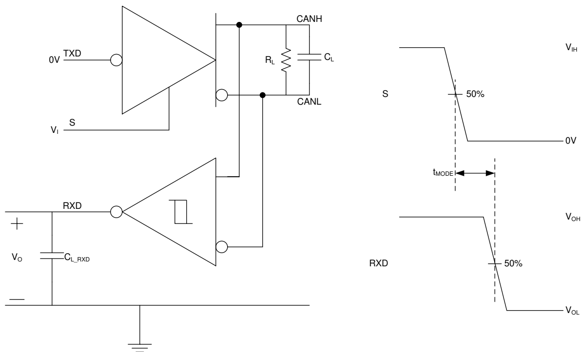
图 7-5. t_{MODE} Test Circuit and Measurement
