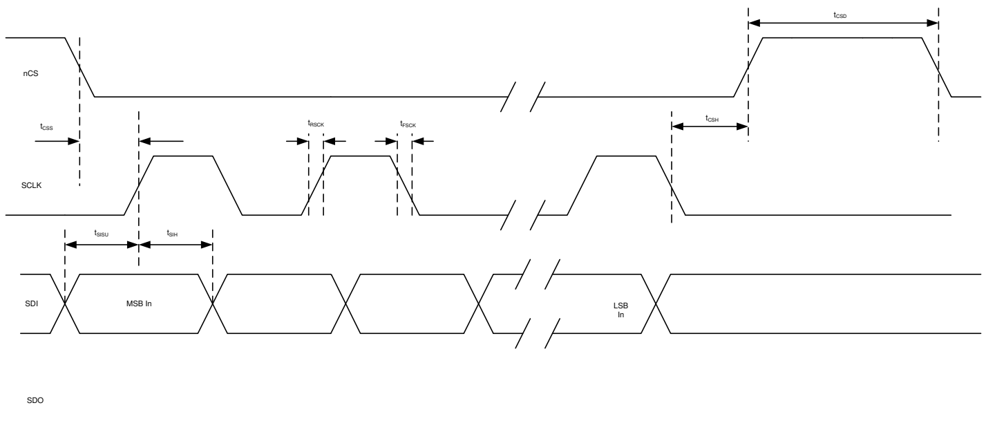
图 7-11. SPI AC Characteristic Write
