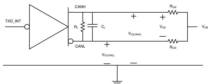
图 7-4. Driver Test Circuit and Measurement
