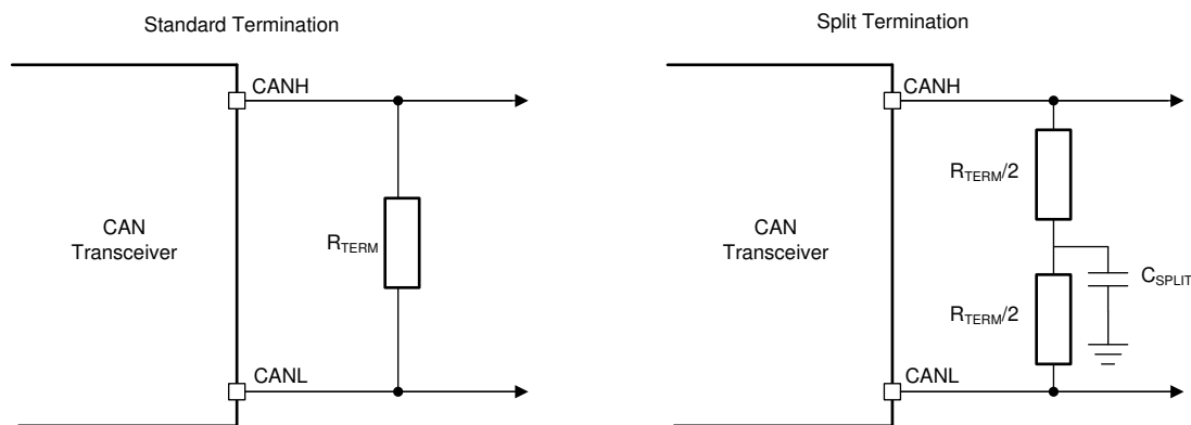
图 9-2. CAN Bus Termination Concepts
