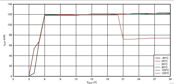
图 9-8. I_{SUP} vs V_{SUP} CAN Dominant with 70 mA Load on V_{CCOUT}
