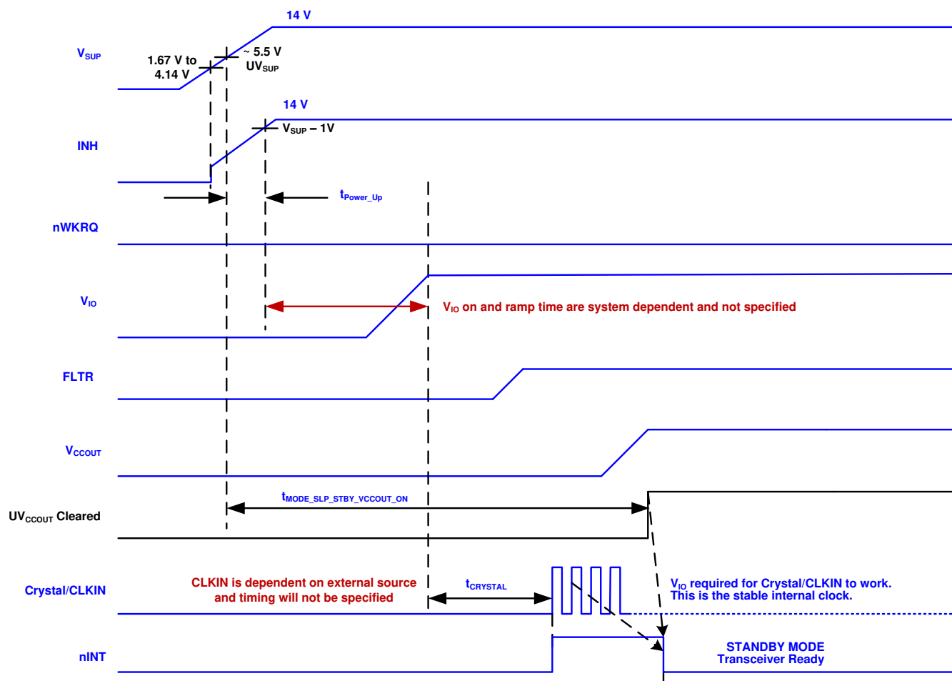
图 7-13. Power Up Timing
