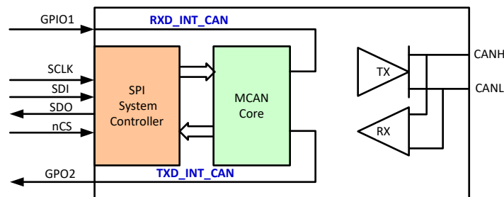
图 8-11. SPI and M_CAN Core Test Mode
