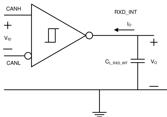
图 7-5. Receiver Test Circuit and Measurement
