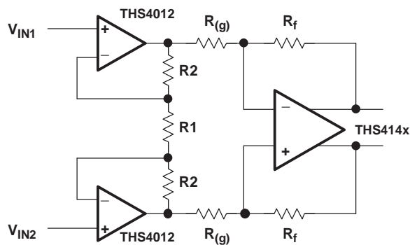
Figure 32. Instrumentation Amplifier
