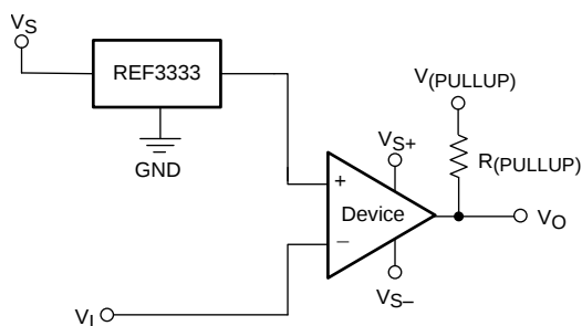
Figure 19. Reference Voltage for the TLV1704-SEP
