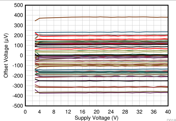
图 6-7. Offset Voltage vs Power Supply
