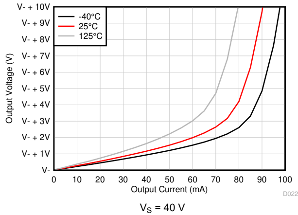
图 6-13. Output Voltage Swing vs Output Current (Sinking)
