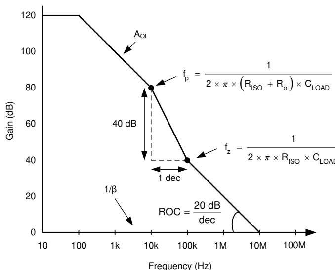
图 8-2. Unity-Gain Amplifier With R_{ISO} Compensation
