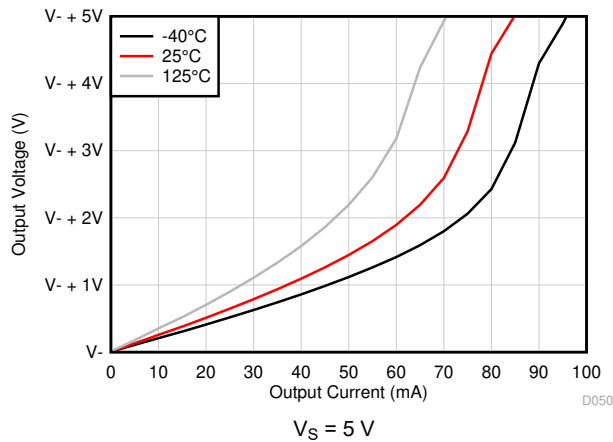
图 6-15. Output Voltage Swing vs Output Current (Sinking)
