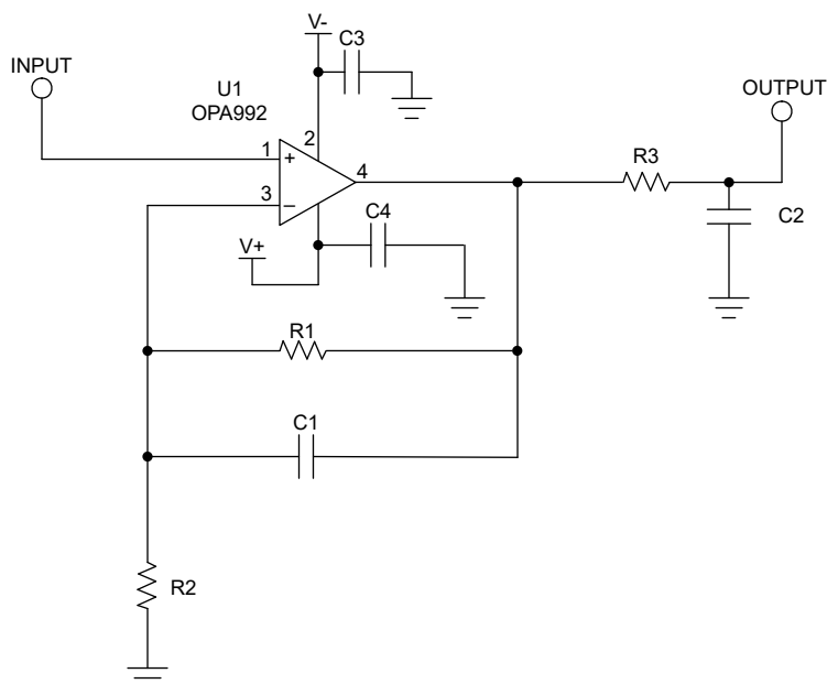
图 10-1. Schematic for Noninverting Configuration Layout Example
