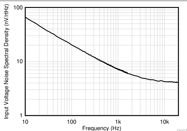
图 6-21. Input Voltage Noise Spectral Density vs Frequency
