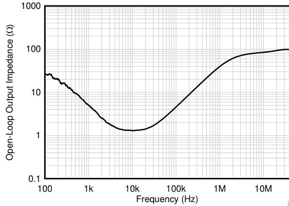
图 6-25. Open-Loop Output Impedance vs Frequency
