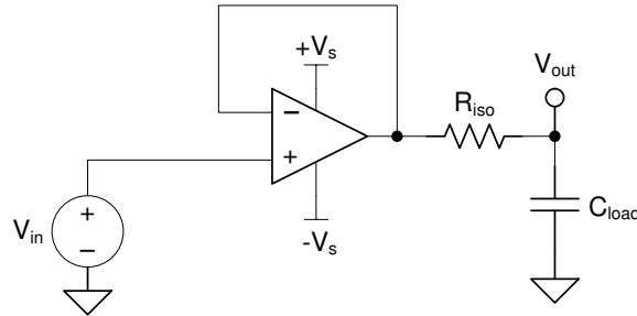
图 7-5. Extending Capacitive Load Drive With the TLV9361
