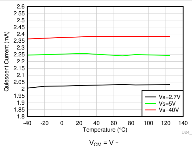
图 6-23. Quiescent Current vs Temperature
