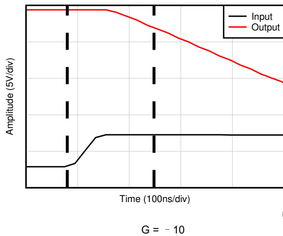
图 6-29. Positive Overload Recovery
