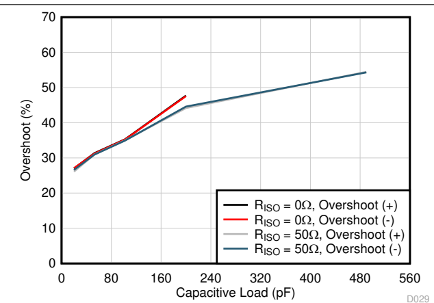
图 7-4. Small-Signal Overshoot vs Capacitive Load (20-mV pp Output Step, G = -1)
