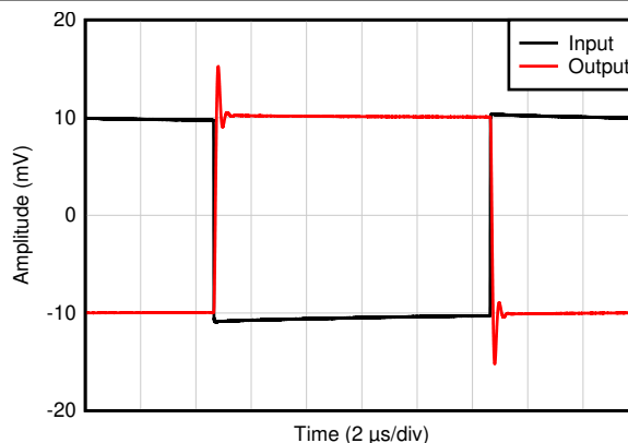
图 6-32. Small-Signal Step Response
