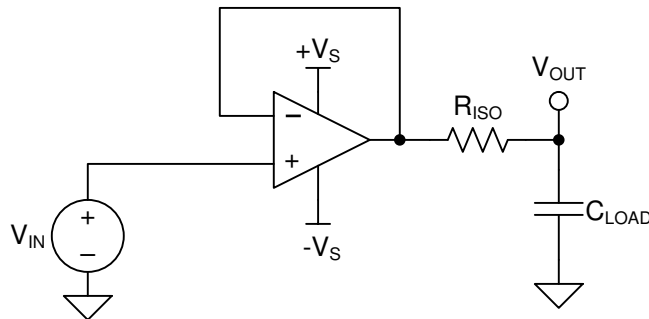
图 8-1. Unity-Gain Buffer With R_{ISO} Stability Compensation
