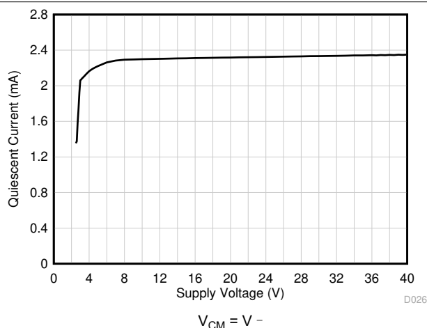
图 6-22. Quiescent Current vs Supply Voltage
