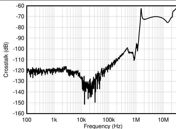
图 6-36. Channel Separation vs Frequency
