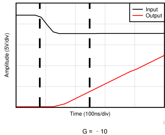
图 6-30. Negative Overload Recovery
