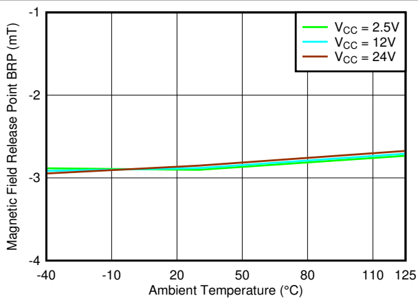
图 7-42. BRP_Z Threshold vs. Temperature
