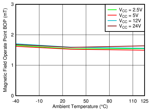
图 7-14. B OP_Y Threshold vs. Temperature
