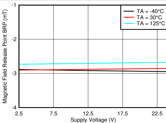
图 7-41. BRP_Z Threshold vs. VCC
