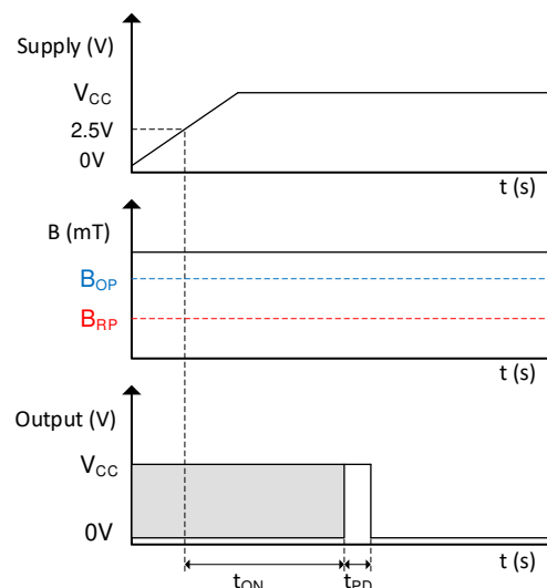
图 8-18. Power-On Time When B > B_{OP}
