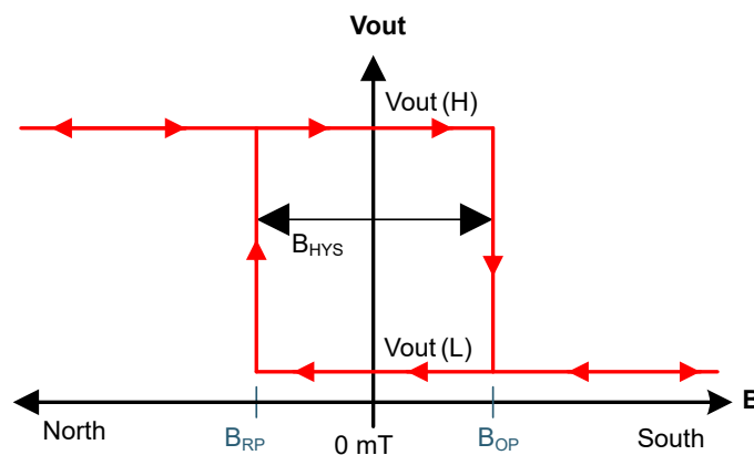
图 8-2. Latch Functionality
