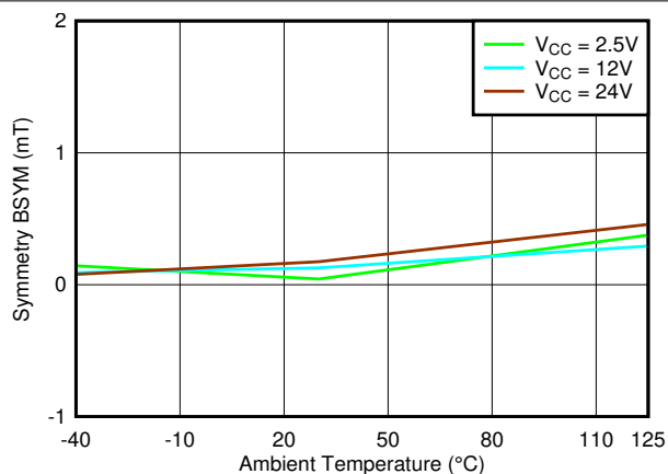
图 7-58. B_{SYM(Z)} vs. Temperature
