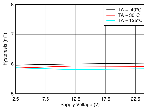
图 7-43. Hysteresis_Z vs. VCC
