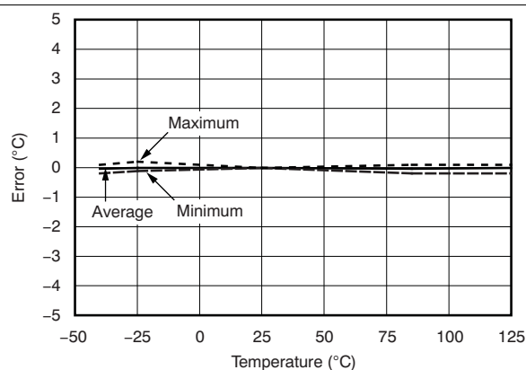
Figure 12. 5^{\circ}C Hysteresis Error vs Temperature
