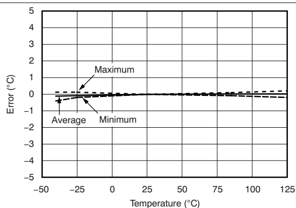
Figure 13. 10^{\circ}C Hysteresis Error vs Temperature
