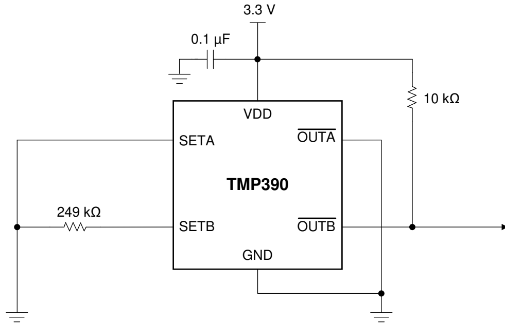
图 8-7. TMP390 One Channel (Cold) Operation Example Circuit With -20^{\circ}\text{C} Trip Point and 10^{\circ}\text{C} Hysteresis
