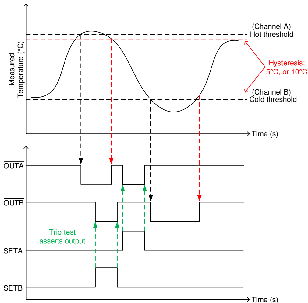
图 7-2. TMP390 Trip Test Operation
