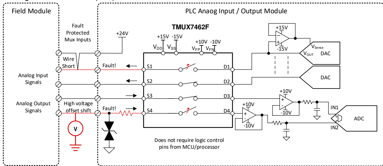
图 9-1. Typical Application
