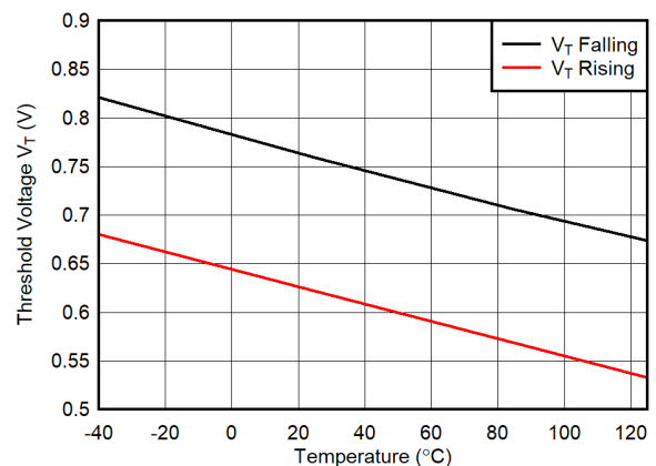
图 6-24. Threshold Voltage vs Temperature
