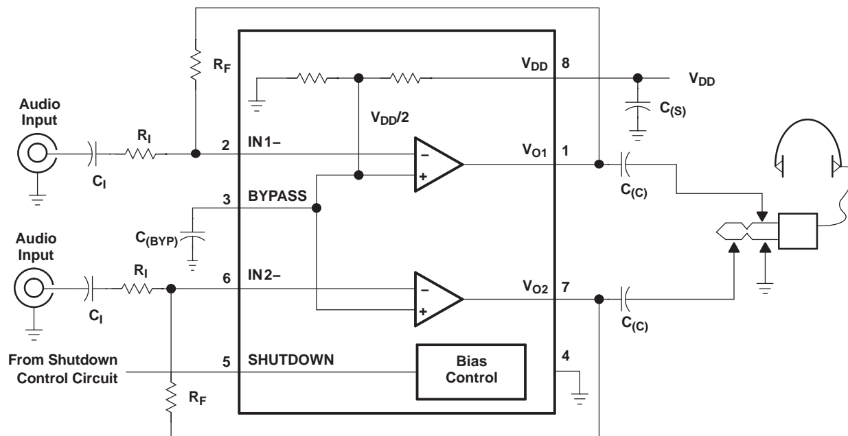
Figure 35. Typical Application
