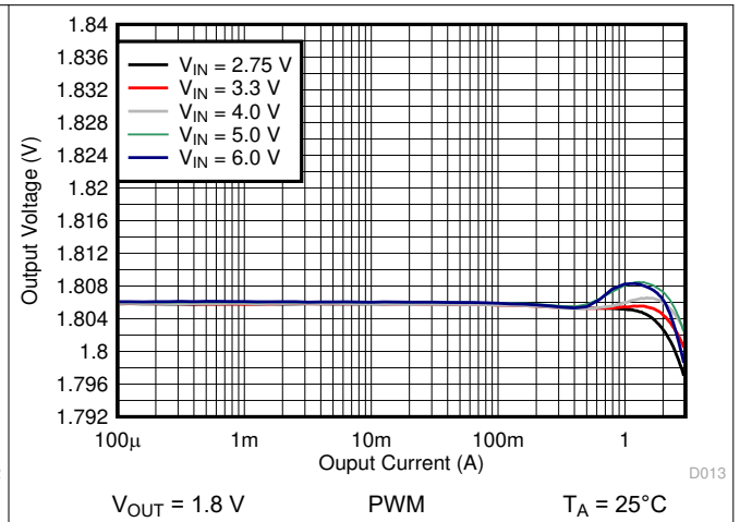
图 10-15. Output Voltage vs Output Current
