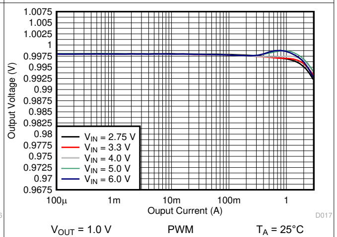
图 10-19. Output Voltage vs Output Current
