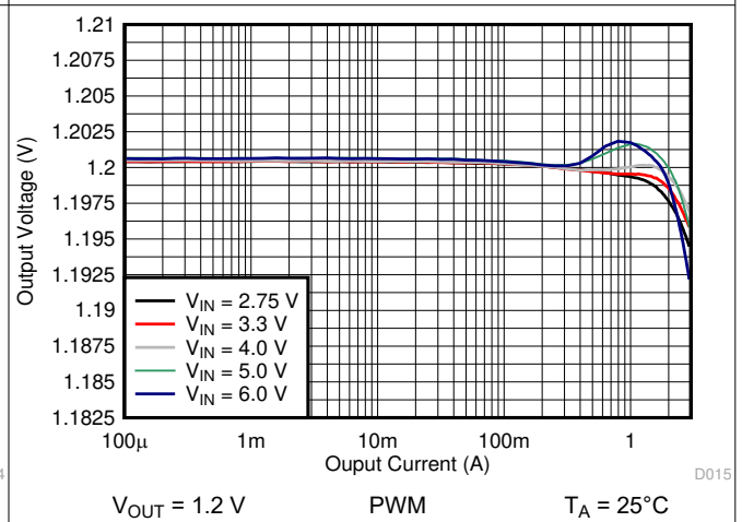
图 10-17. Output Voltage vs Output Current
