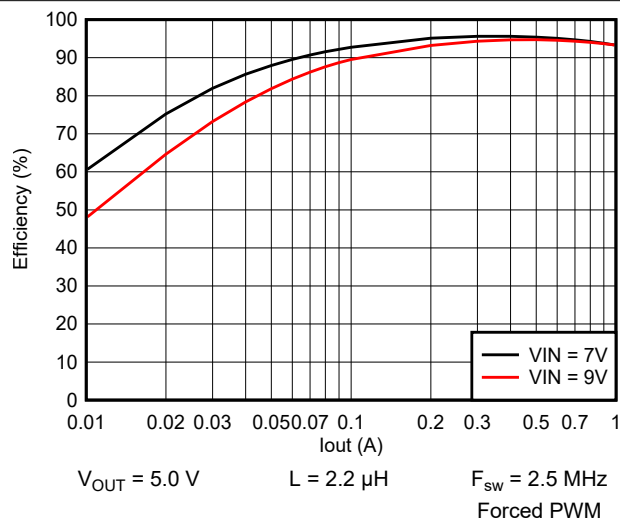
图 9-3. Efficiency vs Output Current
