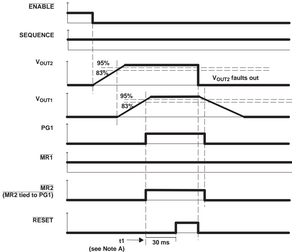
Figure 30. Timing When V_{OUT2} Faults Out
