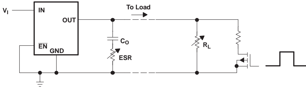
Figure 25. Test Circuit for Typical Regions of Stability
